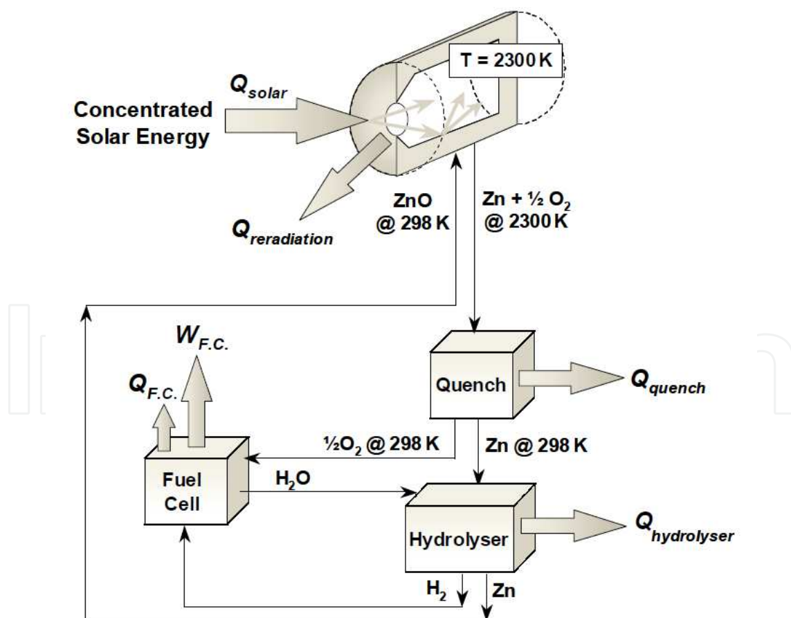
Figure 2. Flowchart for thermochemical hydrogen production from zinc-oxide using concentrated solar energy [5].
