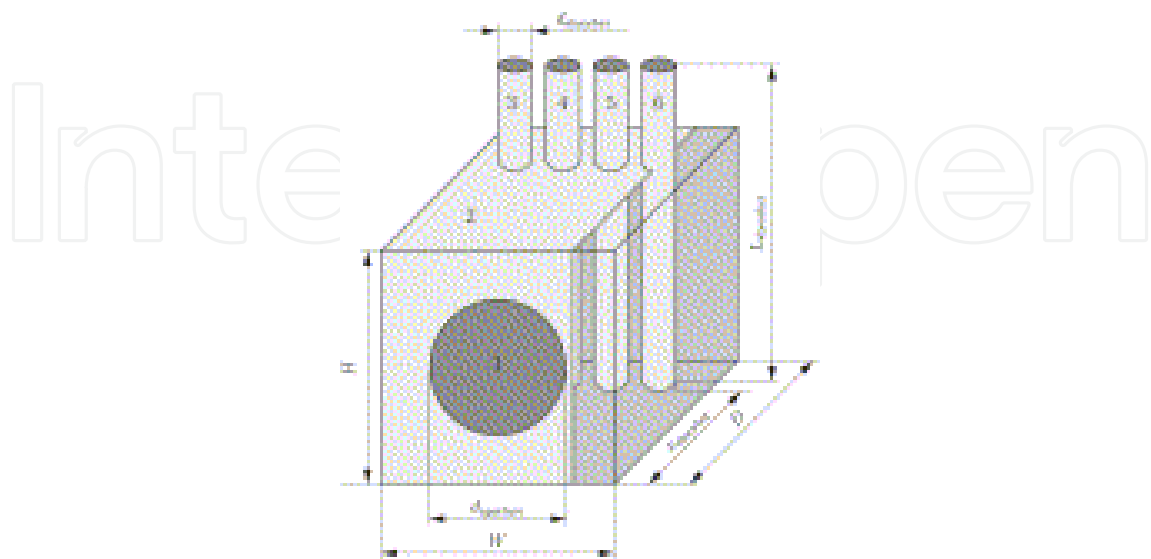
Figure 19. Schematic of design of Maag et al. [72].
