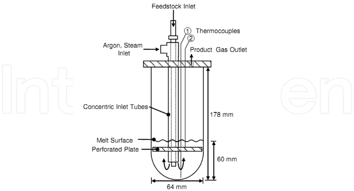
Figure 15. Experimental setup of Hathaway et al. [65].
