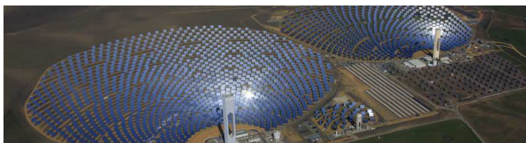
Figure 8. PS 10 (back) and PS 20 (front) solar thermal power plants with heliostats with solar towers [55].
