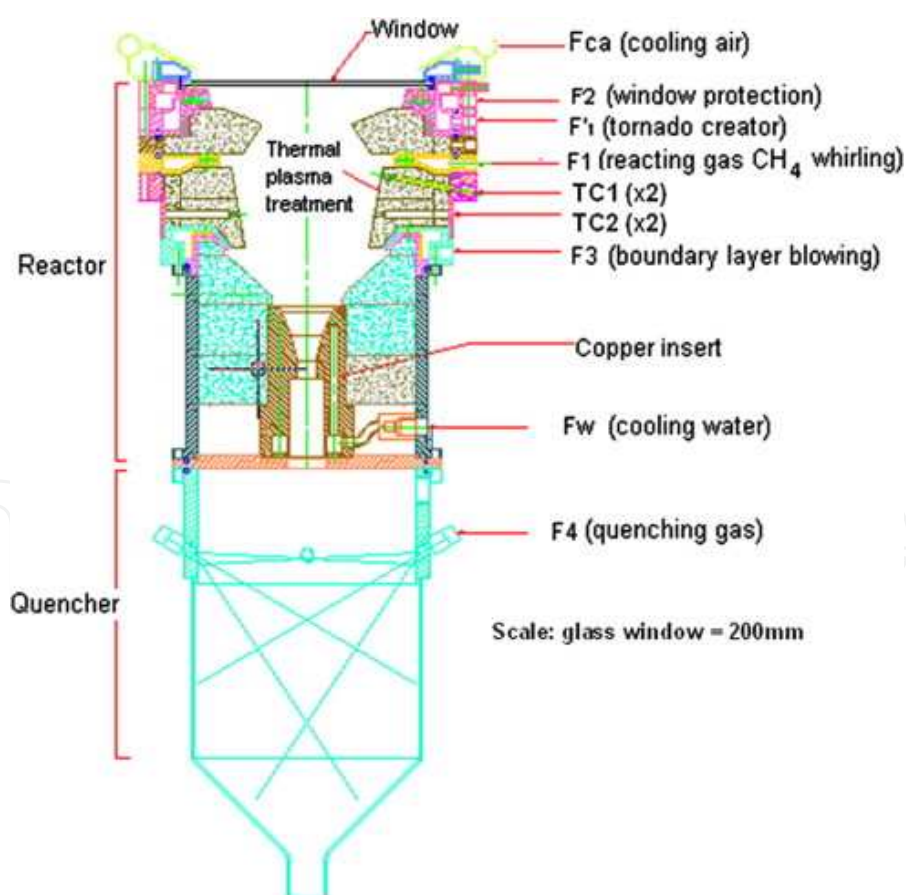
Figure 10. Schematic of design of Yeheskela and Epstein [58].
