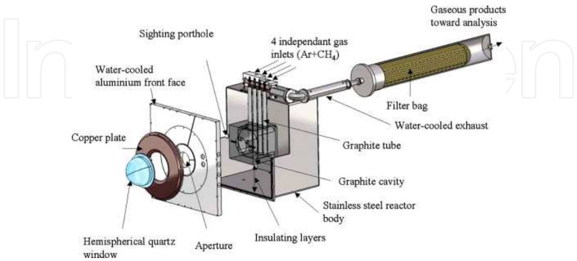
Figure 16. Schematic of design of Rodat et al. [66].
