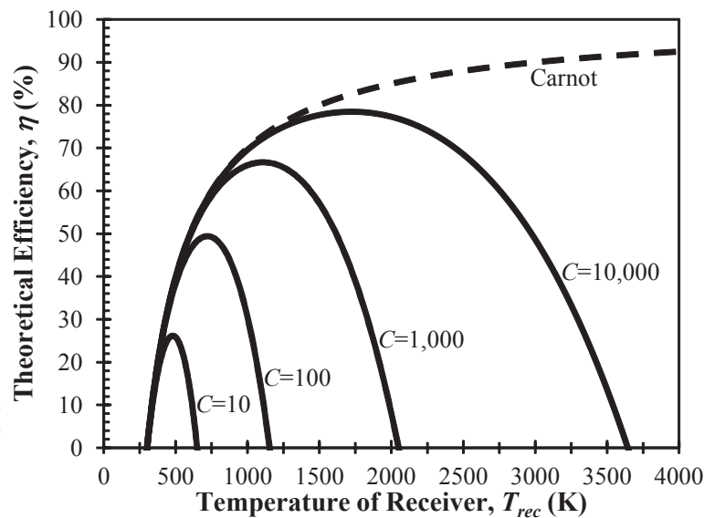
Figure 4. Theoretical solar reactor efficiency, \eta , as a function of receiver temperature, T_{\text{rec}} , for different concentrating ratios, C .
