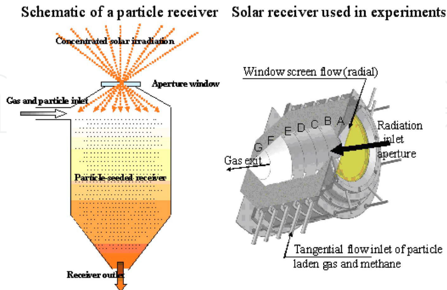
Figure 12. Schematic of design of Klein et al. [61].
