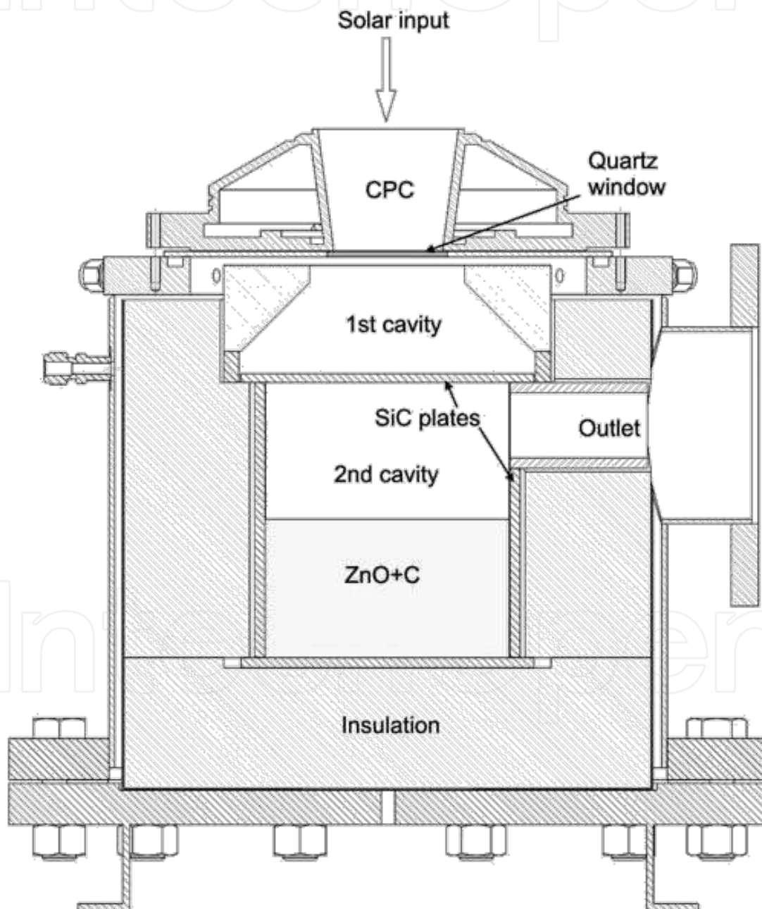
Figure 20. Reactor design of Osinga et al. [73].
