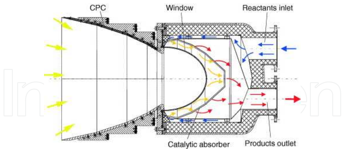
Figure 18. Design of the German Aerospace Center for natural gas reforming [12].
