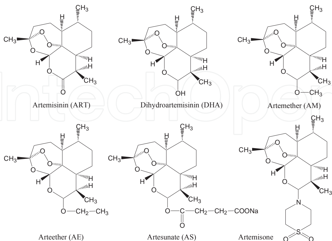
Figure 1. Chemical structures of artemisinin (ART) and its five derivatives, dihydroartemisinin (DHA), artemether (AM), arteether (AE), artesunate (AS) and artemisone
