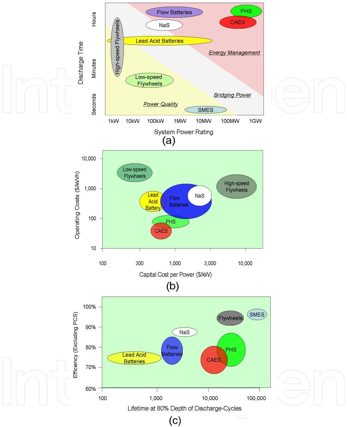
Figure 3. Technical characteristics of CAES
