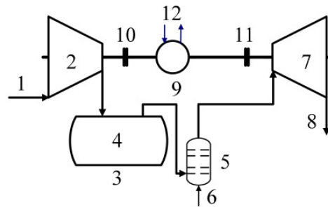
(a) Schematic diagram of GT system
