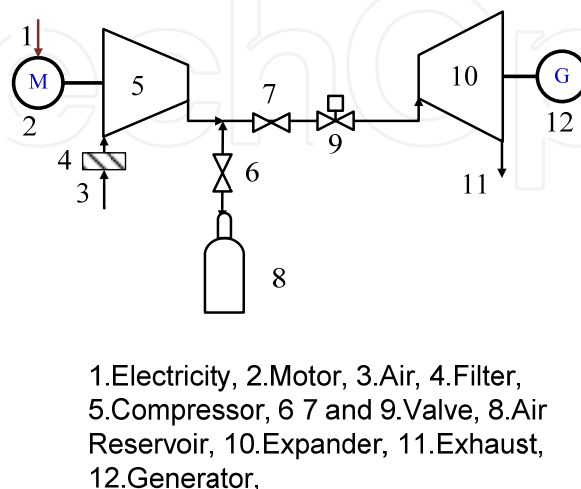
Figure 7. Schematic diagram of the CAES system as a standby power supply
