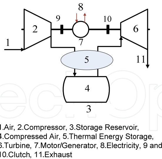
Figure 6. Schematic diagram of AA-CAES system
