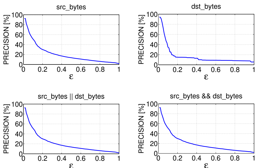
Figure 12. Precision rate.
