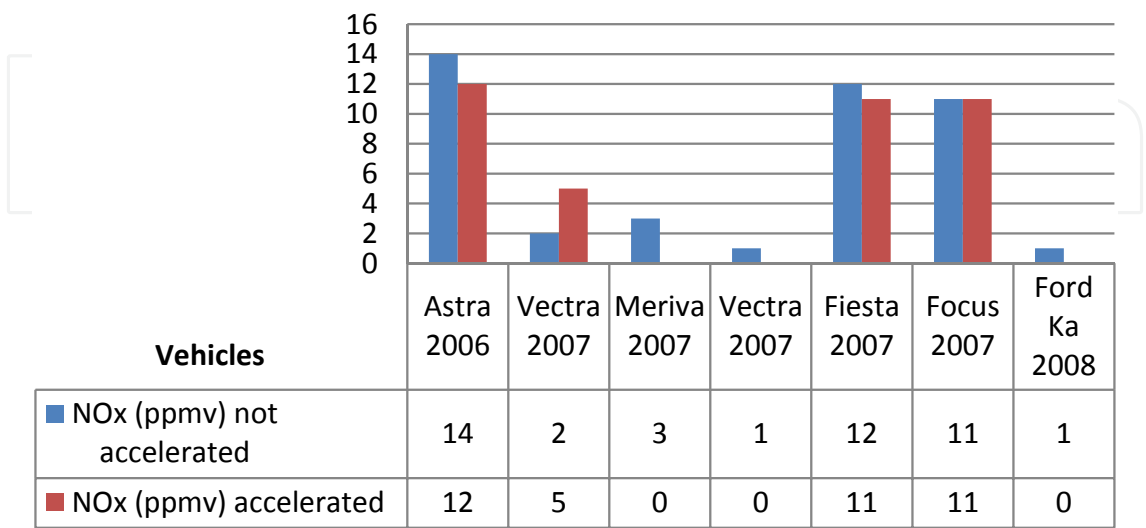
Figure 5. Emission of nitrogen oxides by vehicles using ethanol engine
