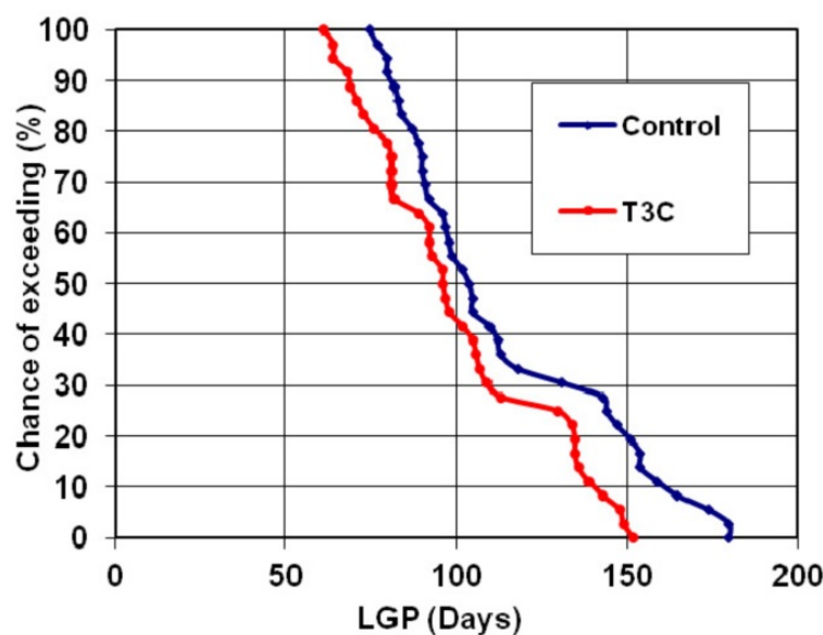
Figure 2. The effect of a 3^{\circ}\text{C} rise in temperature on the Length of Growing Period (LGP) at Makindu, Kenya. 1959-2004 [21]
