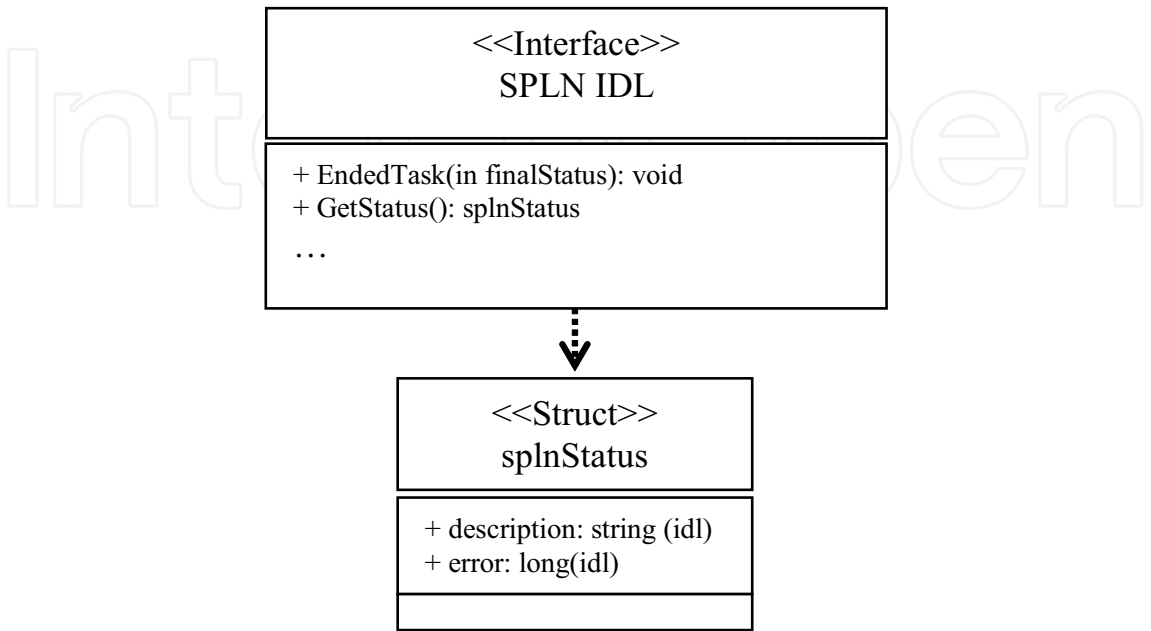
Figure 12. Interface SPLIN
