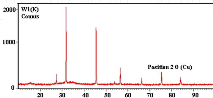
Figure 7. XRD spectrum of GaP nanocrystals prepared on the base of \text{Na}_3\text{P} and \text{GaCl}_3 .
