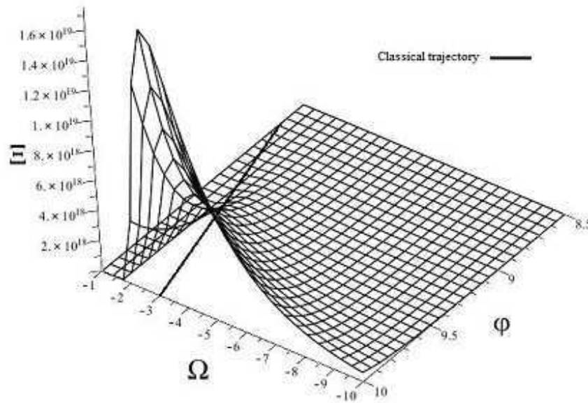
Figure 1. Exact wave function for the free case, i.e. for U(\varphi, \zeta) = 0 . The wave function (66) is peaked around the classical trajectory \Delta\Omega \pm \frac{3}{p}\Delta\varphi = \nu_0 = \text{const} , which is the solid line shown on the \{\Omega, \varphi\} plane. For this case \nu_0 = -1 on equation (68a)
