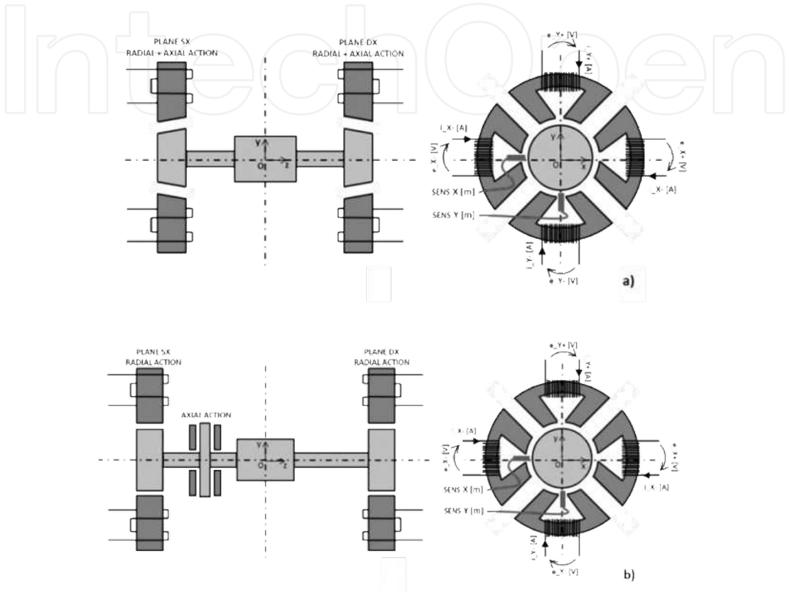
Figure 5. Geometry of actuation stage. a) Conical profile. b) Cylindrical profile.
