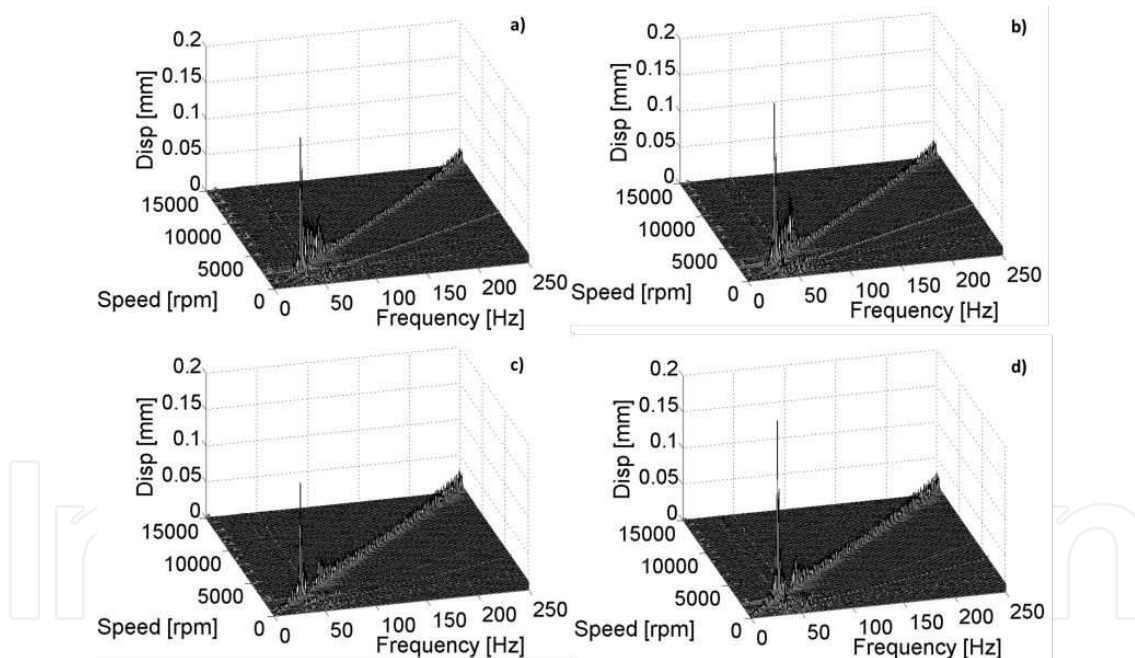
Figure 13. Waterfall plot. a) X1; b) Y1; c) X2; d) Y2.
