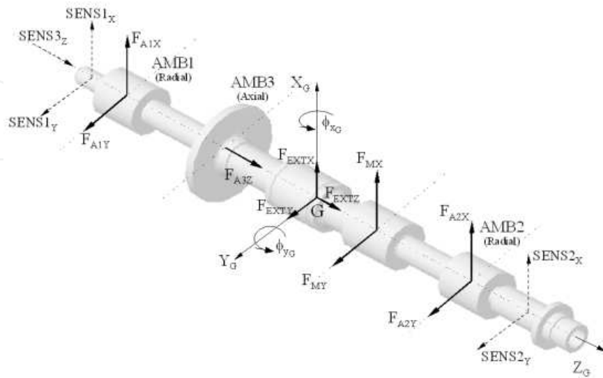
Figure 9. Actuation forces and sensors position.
