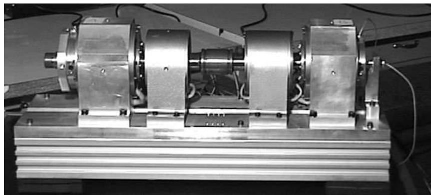
Figure 1. Picture of the rotor.
