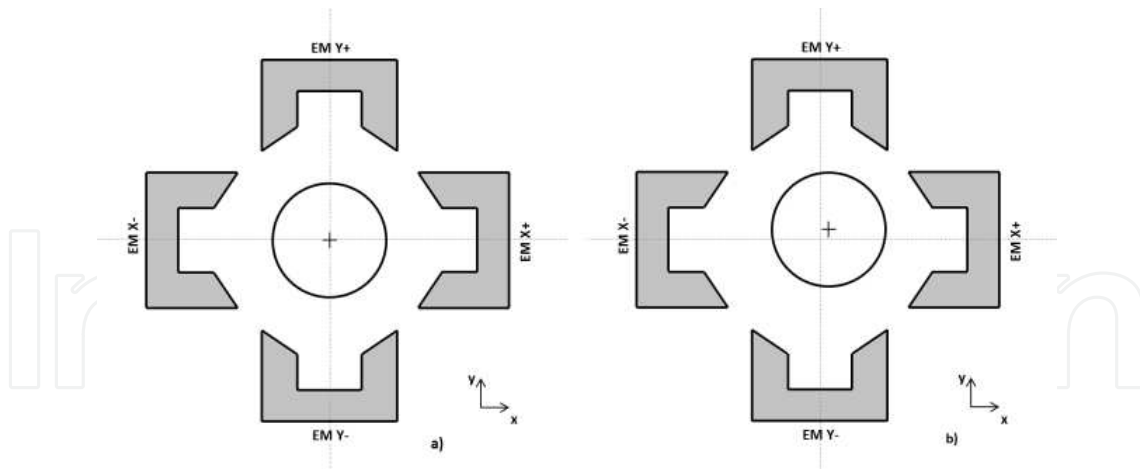
Figure 16. Mechanical centering (a) vs. Electrical centering (b).
