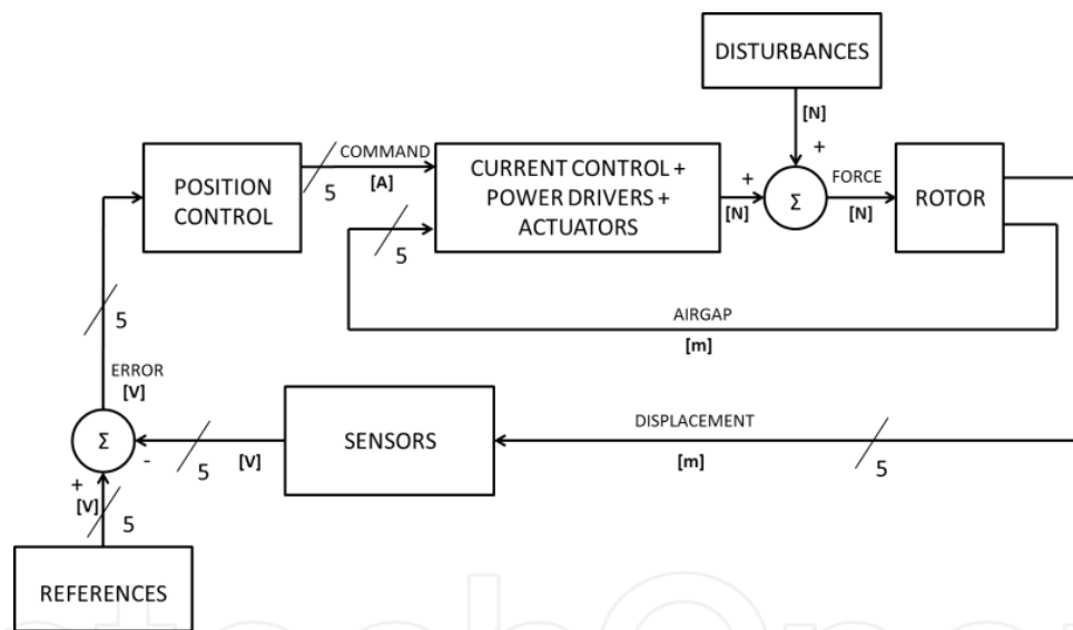
Figure 3. Overall system architecture.
