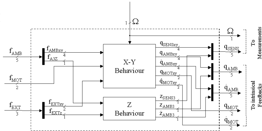
Figure 8. Rotor model block diagram.
