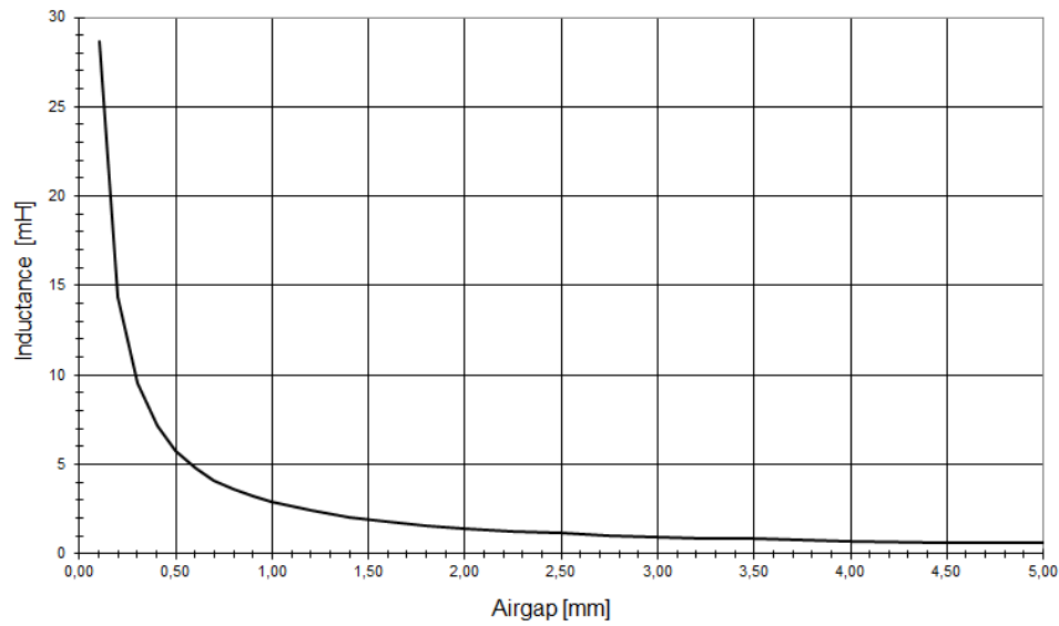
Figure 17. Inductance vs. Position.
