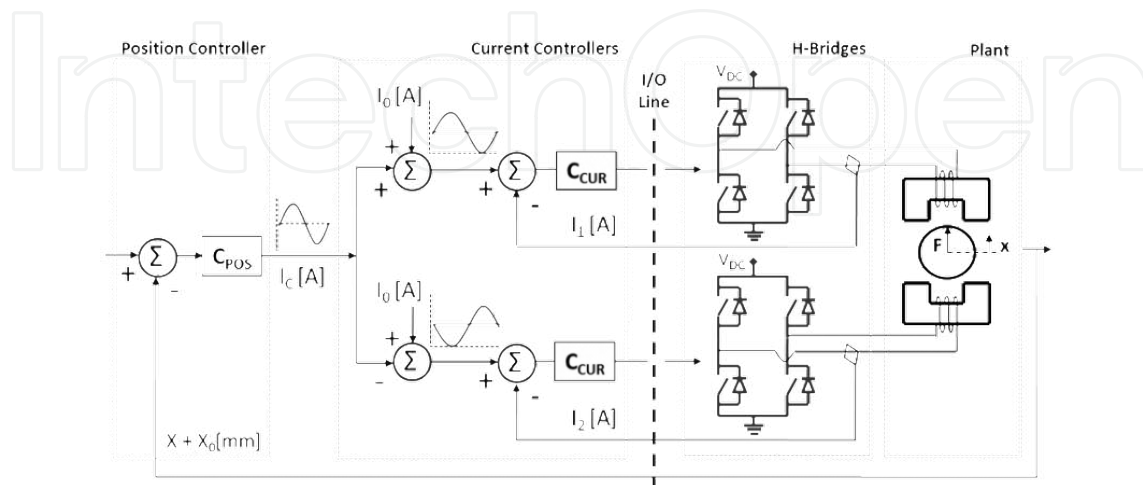
Figure 4. Power driver scheme.
