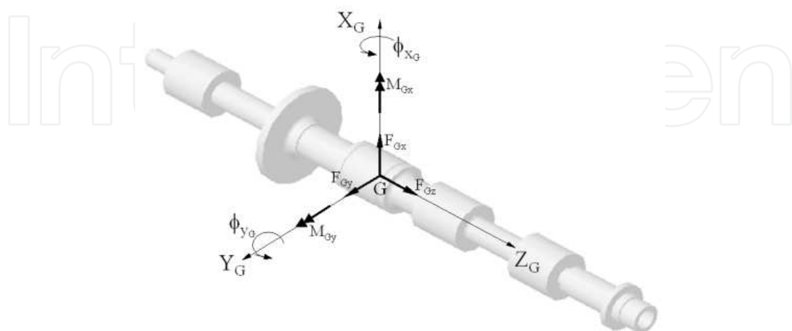
Figure 10. d.o.f. model with generalized displacements and forces.
