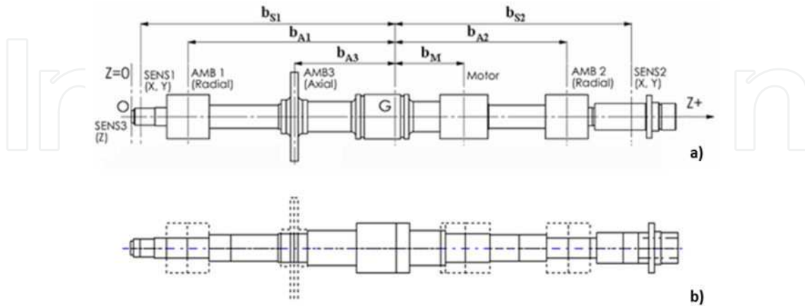
Figure 7. Rotor section view. a) View with dimensions. b) Discretization for FEM modeling.
