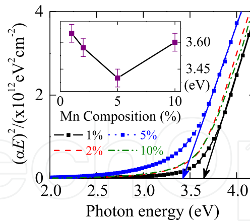
Figure 4. Absorption coefficient vs. incident photon energy near the optical band gap of the BSMT ceramics. The insert is the optical band gap E_g with the different Mn composition. (Figure reproduced with permission from [39]. Copyright 2012, Springer.)
