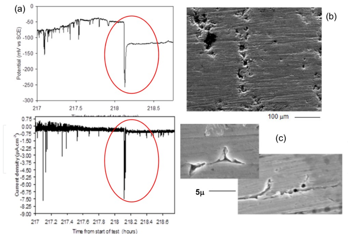
Figure 15. Corrosion pits developed on the stainless steel surface after N=130200 cycles of test in flowing natural seawater. \Delta\sigma = 140 \text{ MPa} ( 58\% \sigma_{0.2} ), after N=130200 cycles, at a load frequency \omega=0.17 \text{ Hz} , stress ratio R=0 , T_{\text{Ave}} = 29^\circ\text{C} and \text{pH}_{\text{Ave}} = 7.9 . (a) Potential and current noise (b) corrosion pits developed on grain boundaries [16] and (c) SEM photomicrograph showing CF small cracks formed at triple point and along grain boundaries.
