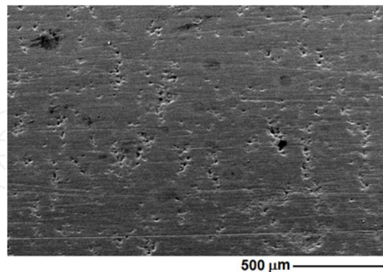
Figure 14. Pits formed at grain boundaries of a 316L SS undergoing cyclic loading in natural seawater. \Delta\sigma = 140 MPa (58% \sigma_{0.2} ), after N=86400 cycles, at a load frequency \omega=0.17 Hz, stress ratio R=0 , T_{Ave}=29^\circ\text{C} and pH_{Ave}=7.9 . Patterns of grain boundaries are revealed practically in the image [56].
