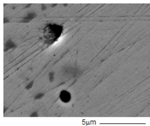
Figure 10. SEM image shows the pits potentiostatically generated in artificial seawater had hemispherical morphology on 316L steel surface under [40].
