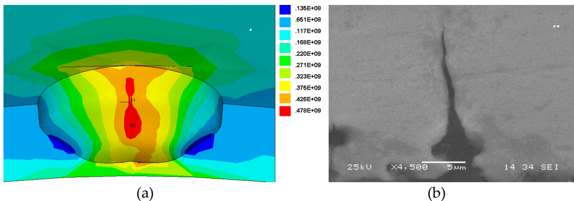
Figure 23. (a) Maximum principal stress distribution at pit contour and (b) small crack emanating from a corrosion pit (Von-Mises: \Delta K_{Isurface}=9.56 \text{ MPa}\sqrt{\text{m}} ; \Delta K_{Ibottom}=7.50 \text{ MPa}\sqrt{\text{m}} ), in a hemispherical shaped pit with a depth= 291 \mu\text{m} and developed on a pressured thin-walled 350 \mu\text{m} tube specimen made of 316L SS; \sigma_{0.02}=241 \text{ MPa} , E=190 \text{ GPa} and \nu=0.33 . The internal pressure and the relation a/c were kept 110 bar and 0.78.
