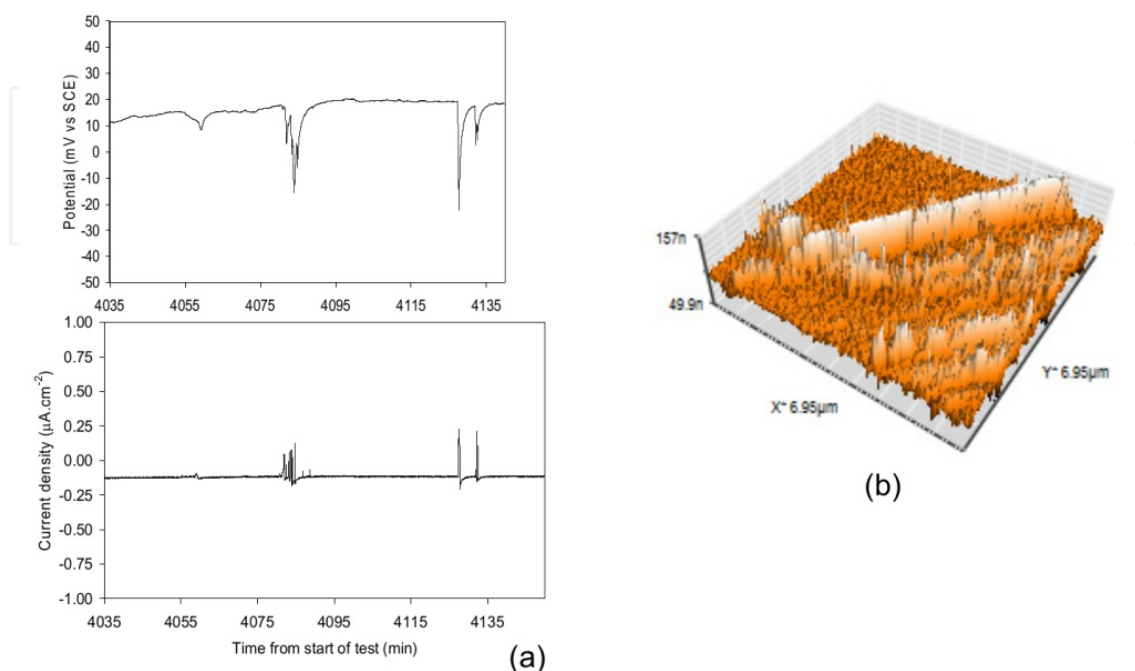
Figure 3. a) Potential and current noise profiles [16] and b) AFM surface image, for a 316L SS exposed to natural seawater under an induced cyclic stress of \Delta\sigma = 140 \text{ MPa} ( 58\%\sigma_{0.2} ), after N=43200 cycles, at a load frequency \omega=0.17 \text{ Hz} and stress ratio R=0 .
