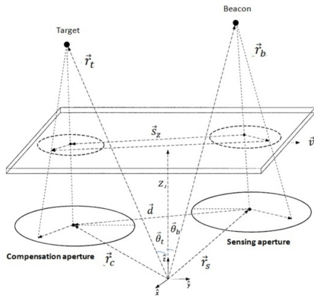
Figure 1. General geometry of the adaptive optical system
