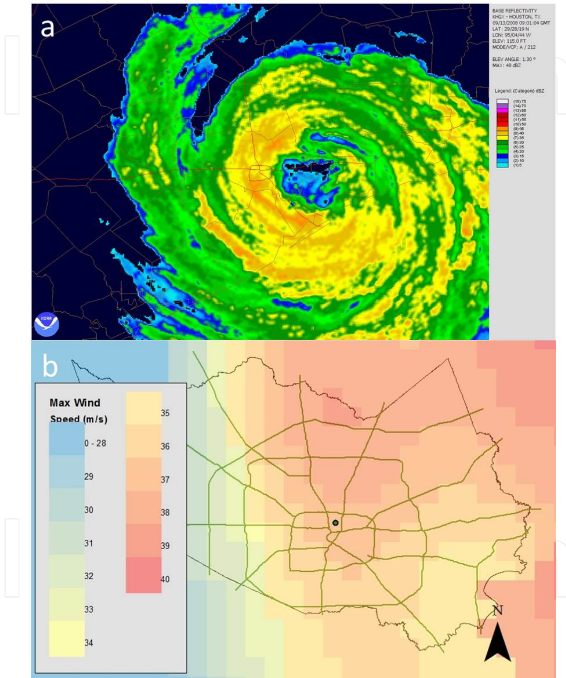
Figure 4. a) Precipitation radar image from 13 September, 09:00 GMT (03:00 CST) overlaid on a Texas county map (grey lines) and including interstate highways (red lines), the circular one in the center depicting Houston's Beltway, which extends for approximately 19 km in its E-W direction. (b) Maximum sustained wind speeds (NOAA Atlantic Oceanographic & Meteorological Laboratory Hurricane Research Division H*Wind product) during Ike in Harris County, Texas, overlaid on the county border (black line) and major thoroughfares (green lines). The central dot marks the tower location.
