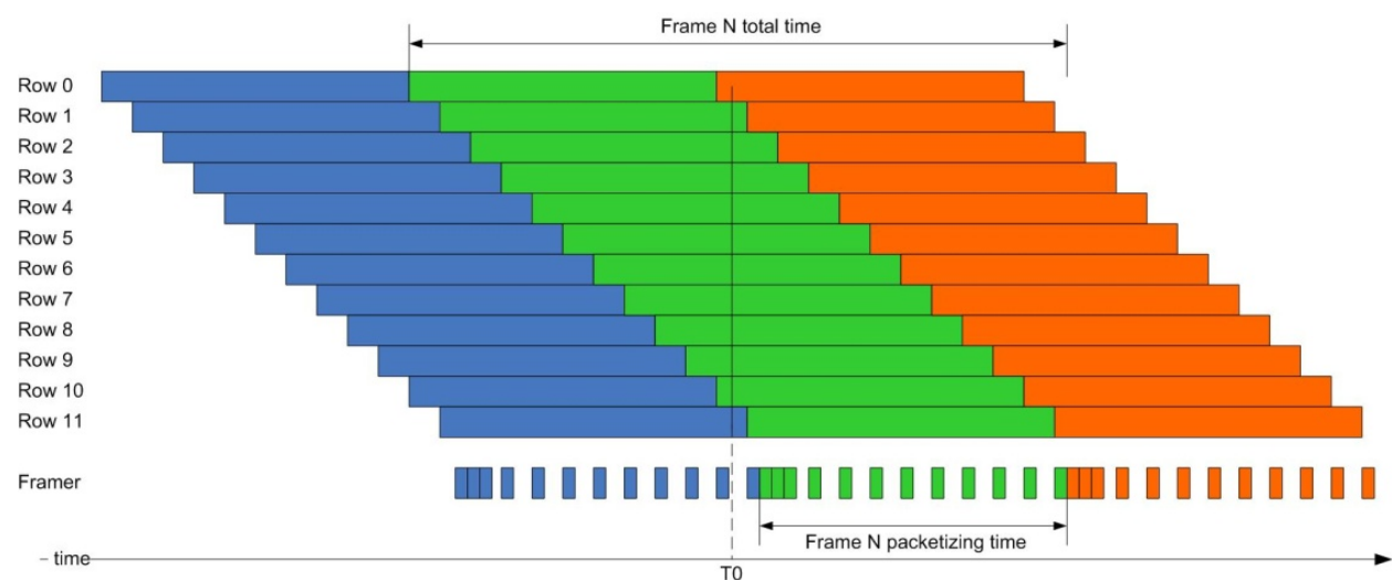
Figure 4. Time Line of Row Processing
