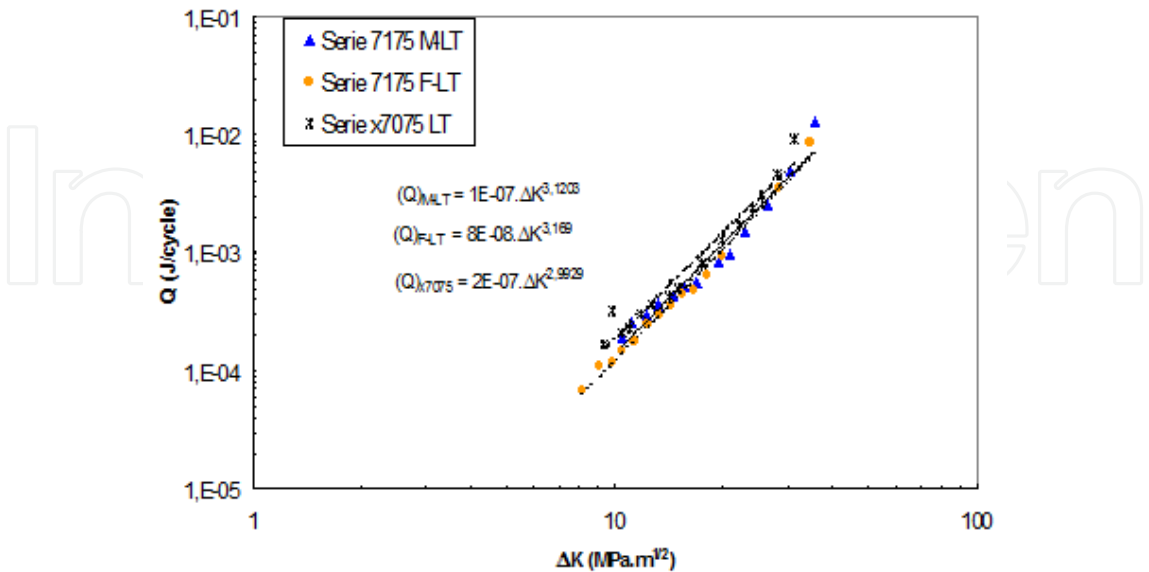
Figure 3. Evolution of energy Q with respect to \Delta K
