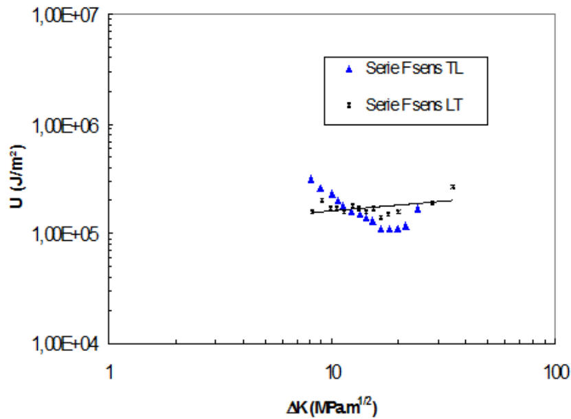
Figure 6. Variation of energy with respect to Δ K for two different orientations (TL and LT)
