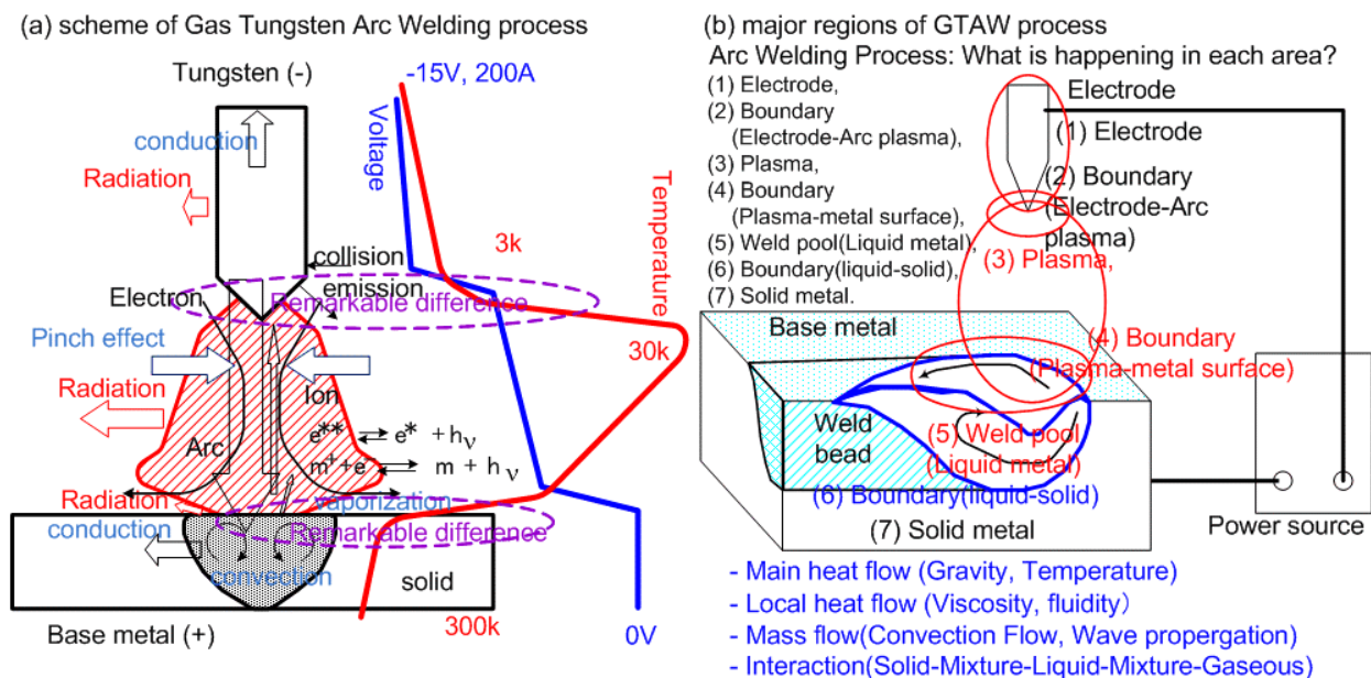
Figure 1. Scheme of Gas Tungsten Arc Welding (GTAW) process.
