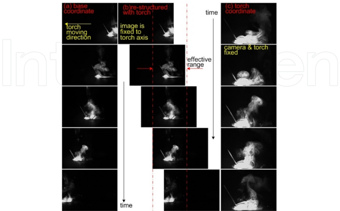
Figure 31. Comparison of coordinate system.
