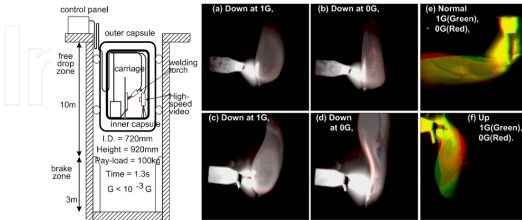
Figure 29. Results of drop tower experiment.
