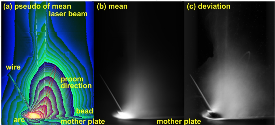
Figure 33. Statistical image of laser arc hybrid welding.
