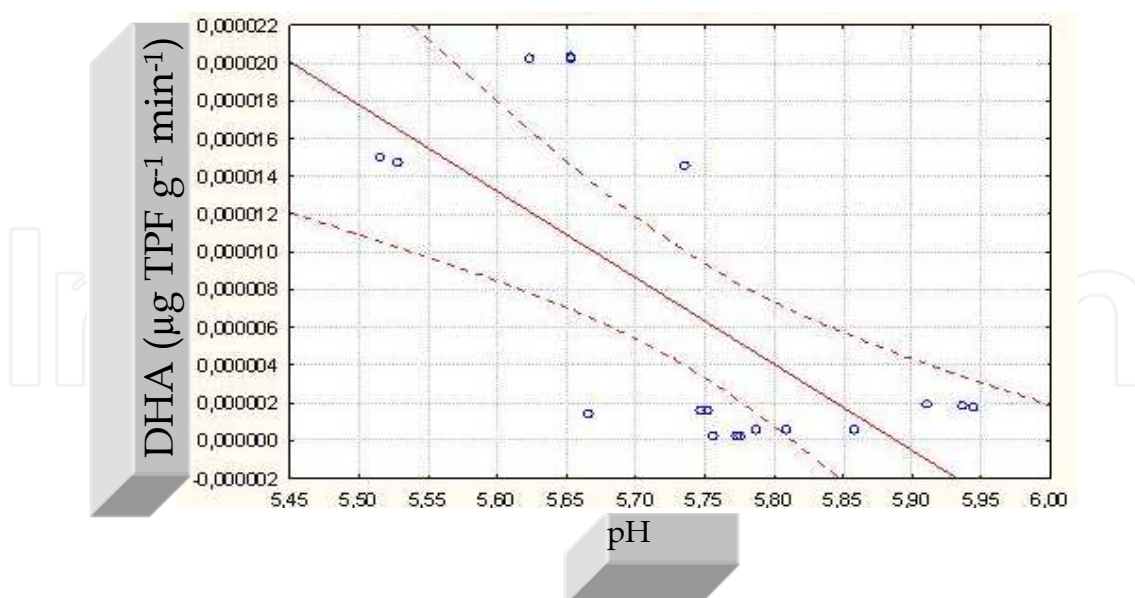
Figure 6. Relationship between DHA and pH values in the Mollic Gleysol ( n=18 , r=-0.70^{**} ), according to Wolińska & Stepniowska (unpublished data)
