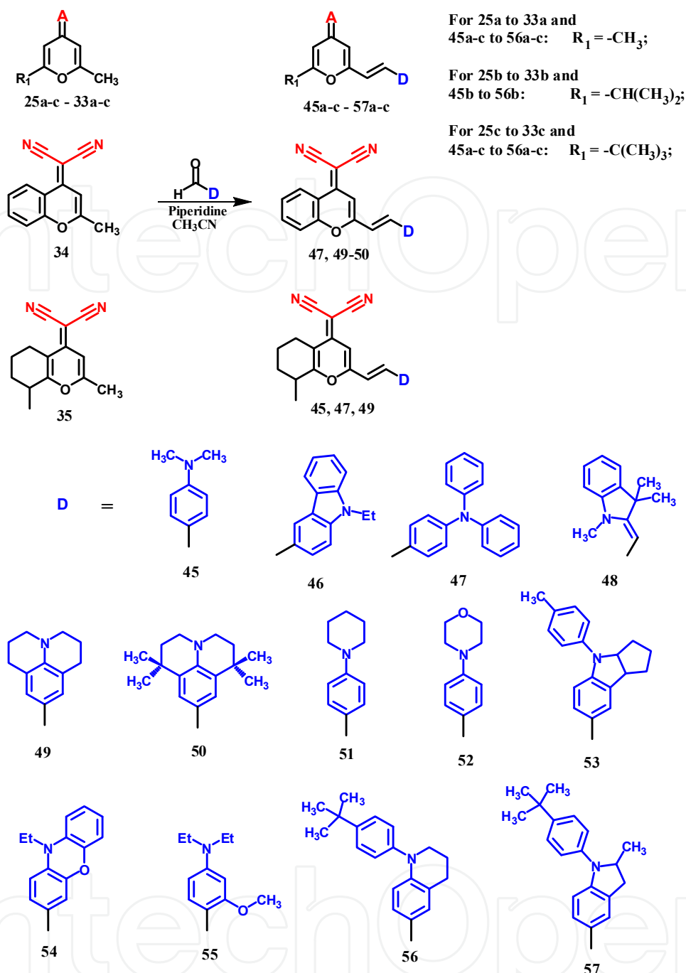
Figure 13. Synthesis of fully functional mono-styryl substituted derivatives of pyranilidene. Electron acceptors are marked in red, electron donors are blue and structure backbone remains in black.
