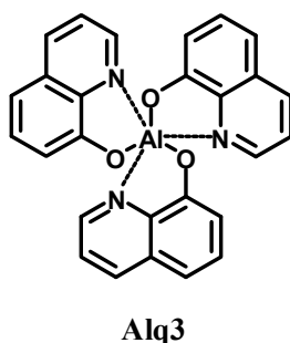
Figure 26. Tris(8-hydroxyquinolato)aluminium ( Alq 3 ) is a well known light-emitting material.
