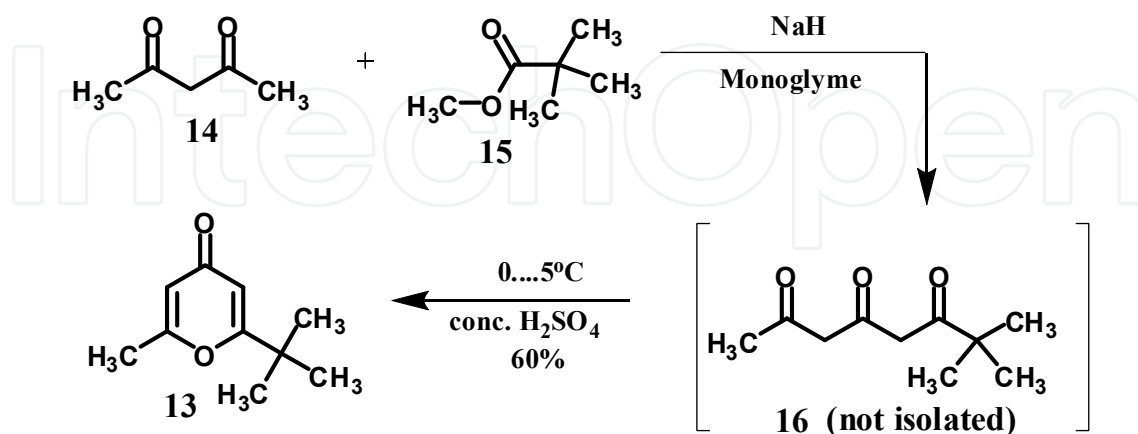
Figure 5. Improved synthesis of 2- tert -butyl-6-methyl-4 H -pyran-4-one (compound 13 ). NaH - sodium hydride, conc. \text{H}_2\text{SO}_4 - concentrated sulfuric acid.
