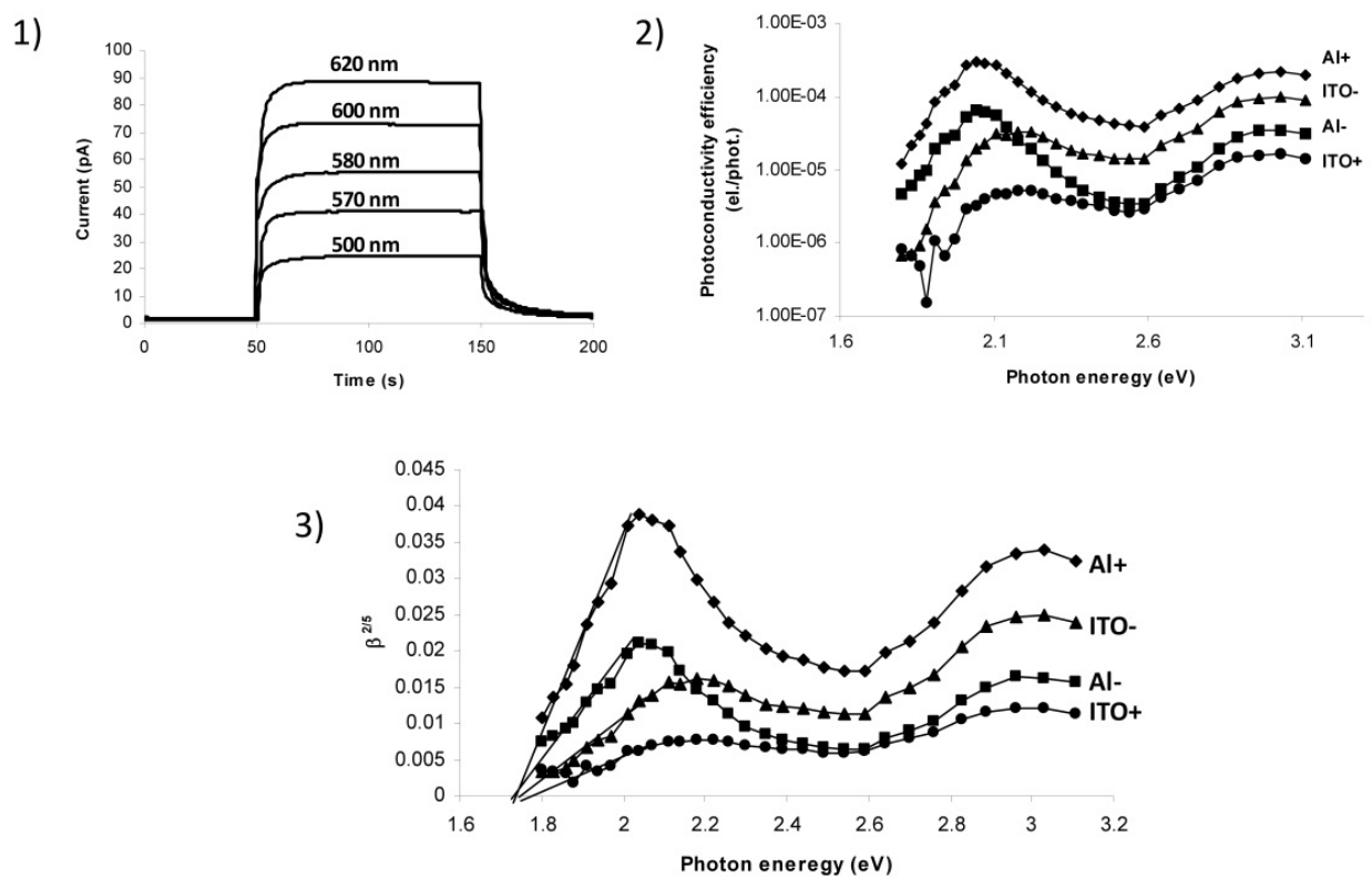
Figure 29. 1) Photocurrent at different wavelength for JWK-2 compound ,2) Dependency of photoconductivity efficiency on photon energy for JWK-2 compound,3) Determination of E_{th} from photoconductivity efficiency spectral dependence.
