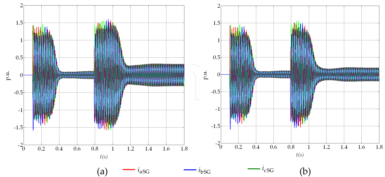
Figure 16. Stator current ( i_{abcSG} ) of the grid (synchronous generator), during sudden change load: a) impact load b) load disconnected
