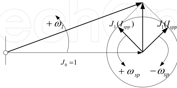
Figure 2. Vector representation of PM for broken bars
