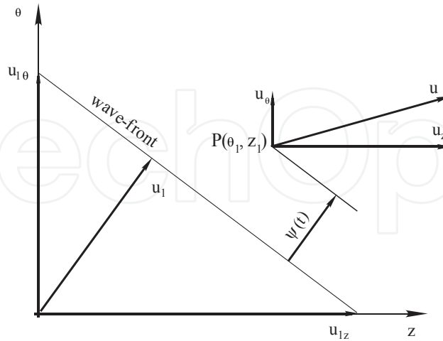
Figure 6. Rotary-linear slip derivation (Mendrela et al., 2003).
