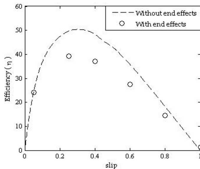
Figure 29. Characteristic of efficiency vs linear slip.
