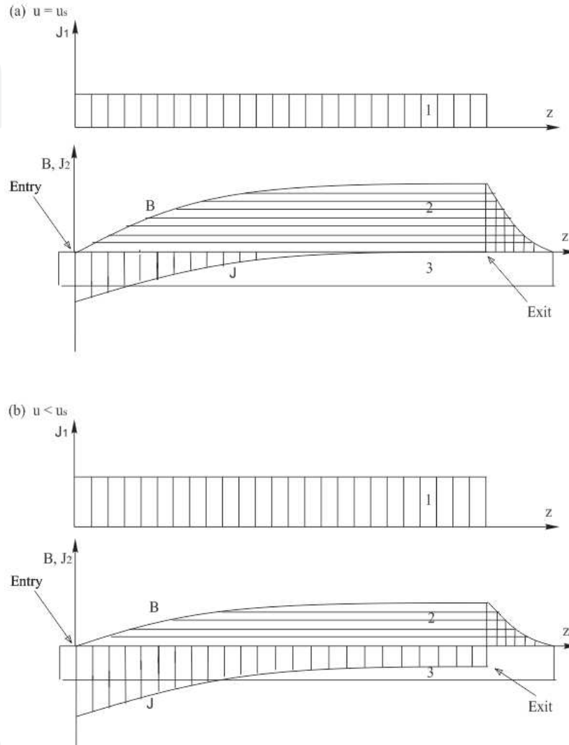
Figure 16. Distribution of primary current ( J_1 ), secondary current ( J_2 ) and magnetic flux density in the air-gap ( B ): (a) u = u_s (b) u < u_s .
