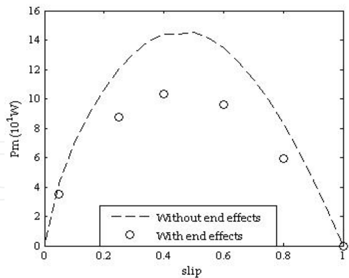
Figure 28. Characteristic of output power vs linear slip.
