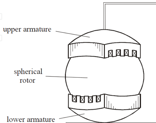
Figure 3. Construction scheme of twin-armature induction motor with spherical rotor (Mendrela et al., 2003).
