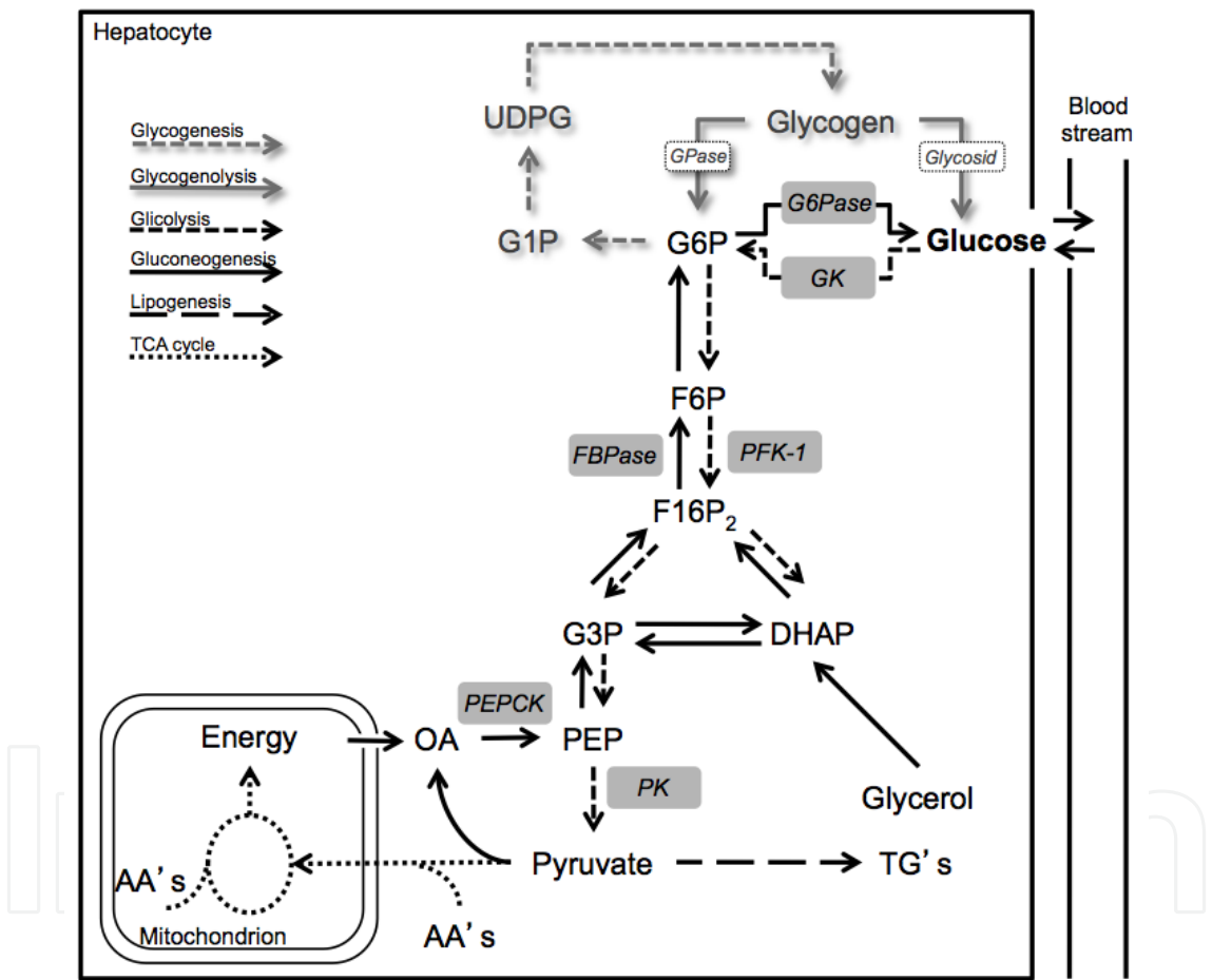
Figure 1. Metabolic model representing main pathways in the liver involving catabolism and anabolism of glucose. Gluconeogenic precursors are represented by pyruvate (and gluconeogenic amino acids, metabolized via the anaplerotic pathways of TCA cycle) as well as glycerol from lipolysis. Some metabolic intermediates were omitted for clarity. Abbreviations are as follows: G6P - glucose 6-phosphate; G1P - glucose 1-phosphate; UDPG - uridine diphosphoglucose; F6P - fructose 6-phosphate; F16P 2 - fructose-1,6-bisphosphate; G3P - glyceraldehyde 3-phosphate; DHAP - dihydroxyacetone phosphate; PEP - phosphoenolpyruvate; TG's - triglycerides; OA - oxaloacetate; AA's - amino acids; GK - glucokinase; G6Pase - glucose-6-phosphatase; FBPase - fructose biphosphatase; PFK-1 - 6-phosphofructo-1-kinase; PEPCCK - phosphoenolpyruvate carboxykinase; PK - pyruvate kinase; GPase - glycogen phosphatase; Glycosid - glycosidic enzymes; TCA cycle - tricarboxylic acid cycle.
