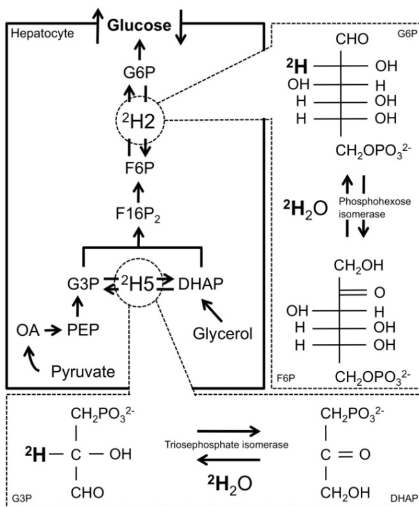
Figure 2. Metabolic model representing gluconeogenesis in the liver with special detail to the labeling with deuterium in position 2 ( 2 H 2 ) and 5 ( 2 H 5 ) of the glucose molecule. Some metabolic intermediates were omitted for clarity. Abbreviations are as follows: G6P - glucose 6-phosphate; F6P - fructose 6-phosphate; F16P 2 - fructose 1,6-bisphosphate; G3P - glyceraldehyde 3-phosphate; DHAP - dihydroxyacetone phosphate; PEP - phosphoenolpyruvate; OA - oxaloacetate; 2 H 2 O - deuterated water.
