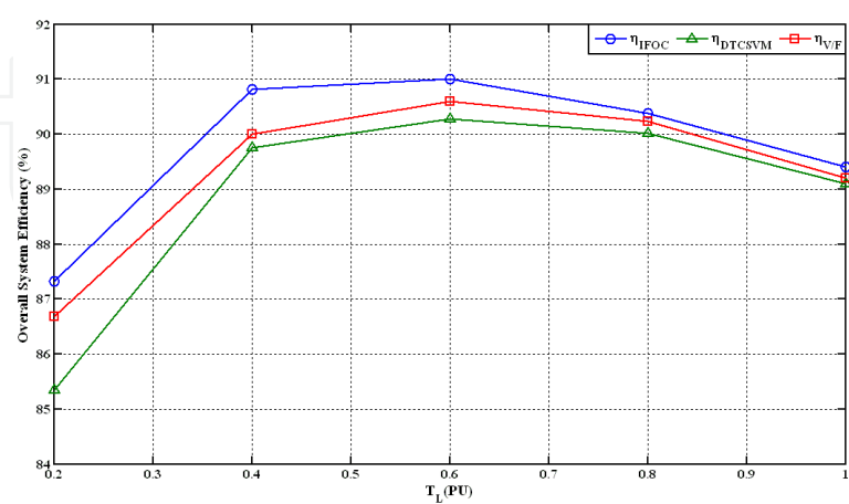
Figure 21. Overall system efficiency at different load torque values
