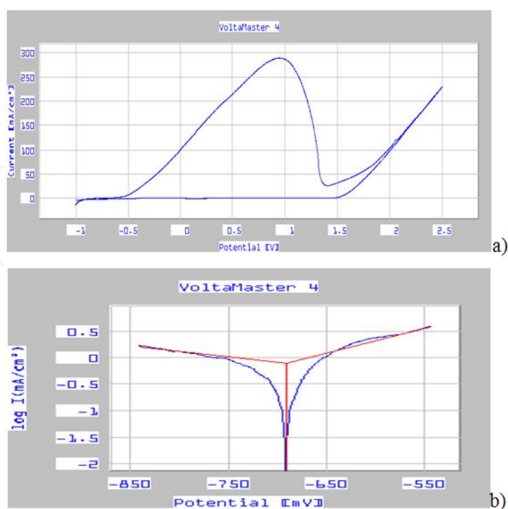
Figure 2. Uncoated carbon-steel electrode; 20% \text{Na}_2\text{SO}_4 support electrolyte; polarisation speed – 100 mV/s; 25°C temperature. a – cyclic voltammogram; b – Tafel test
