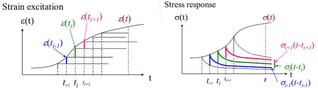
Figure 6. Generalized strain excitation and the stress response of viscoelastic materials to the former. From the relationship between the excitation and the response, Boltzmann's equation, eq. 7, was derived.
