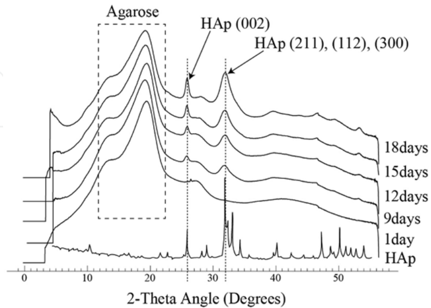
Figure 11. X-ray diffraction profiles for cell-seeded agarose gel cultured for indicated days. That for HAp powder is also shown for reference (Okasaki et al., 1997). (From Hanazaki et al., J. Biorheology. In press. DOI 10.1007/s12573-011-0043-2. With permission.)
