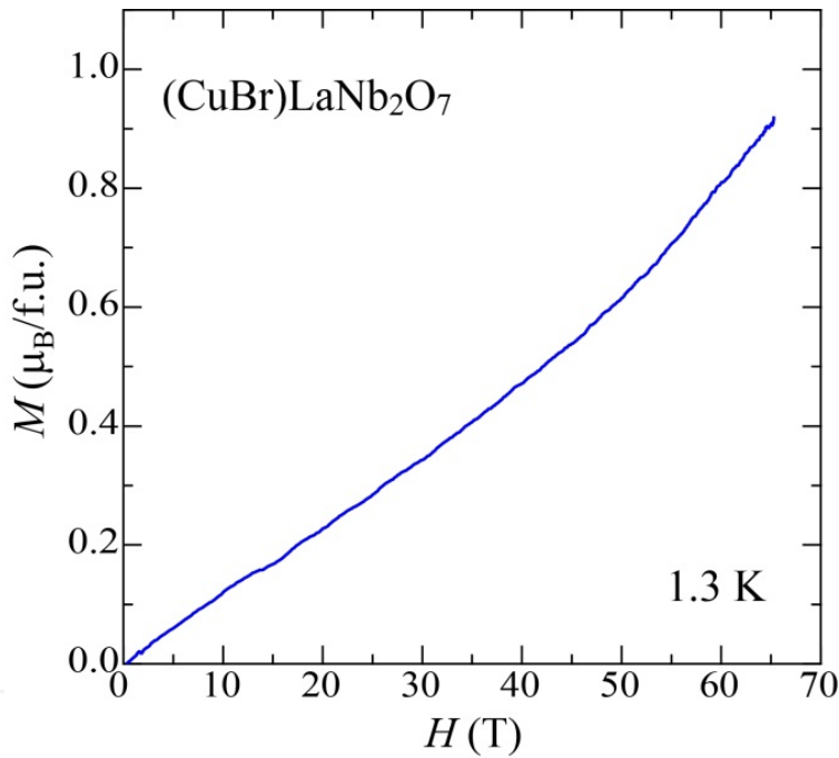
Figure 11. High-field magnetization for (\text{CuBr})\text{LaNb}_2\text{O}_7 at 1.3 K [37].
