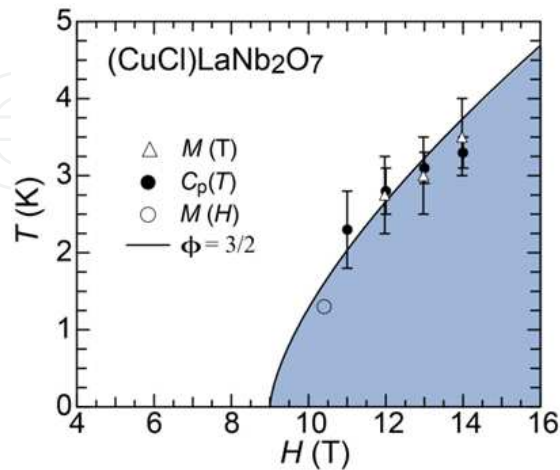
Figure 7. Phase boundary between spin-singlet state and the BEC state in (\text{CuCl})\text{LaNb}_2\text{O}_7 determined from the results of M(T) , M(H) , and C_p(T) . The solid line represents a theoretical curve described in the text [29].
