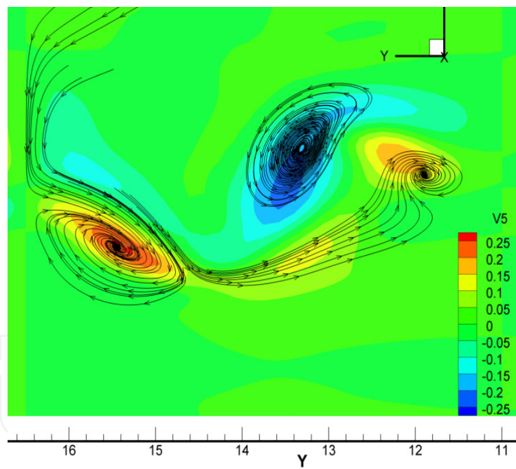
Figure 17. Stream traces velocity vector around ringlike vortex
