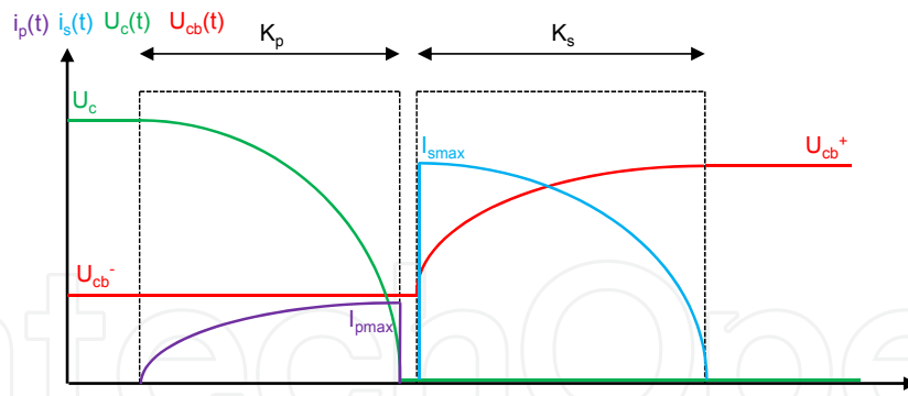
Figure 48. Voltages and currents during power conversion
