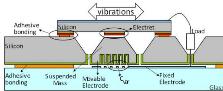
Figure 27. IMEC's first electret-based vibration energy harvester [32]
