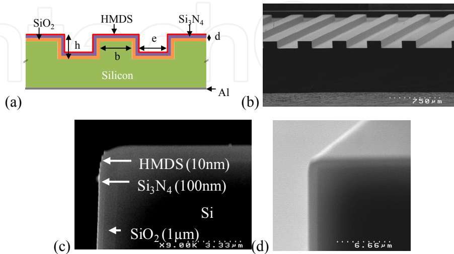
Figure 38. Patterned \text{SiO}_2/\text{Si}_3\text{N}_4 electrets from CEA-LETI [51]
