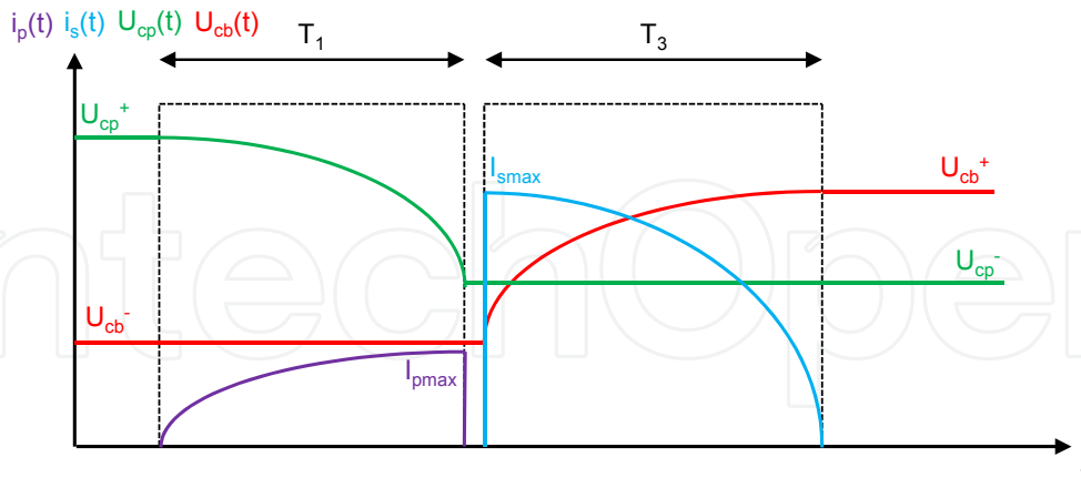
Figure 51. Voltages and currents during power conversion
