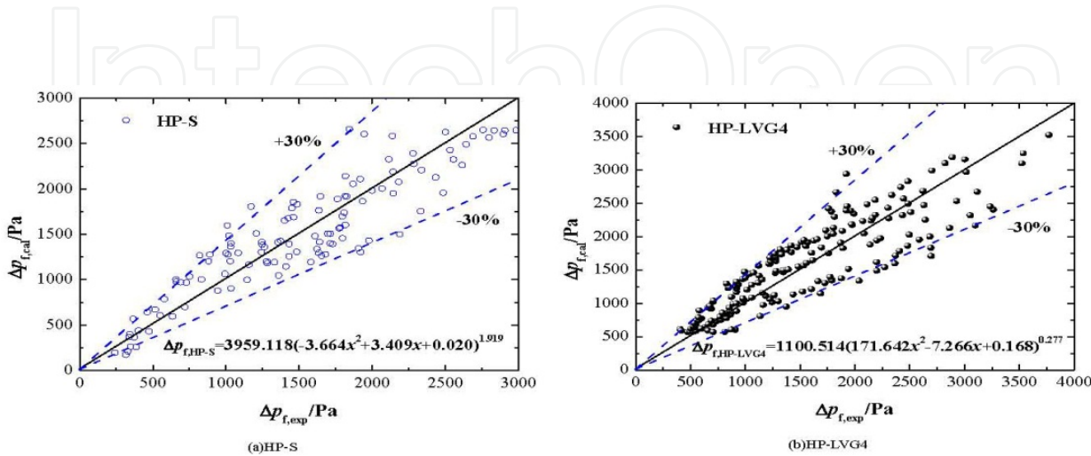
Figure 18. Friction pressure drop comparison between prediction and experiment in the two cases.
