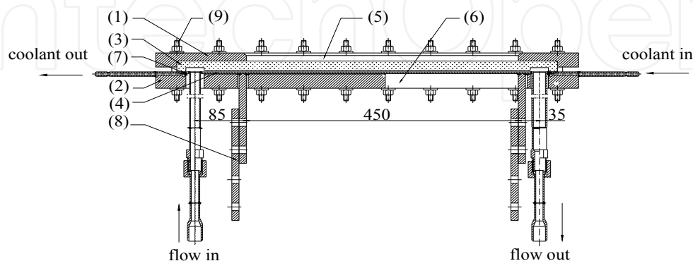
(1) upper holder (2) lower holder (3) quartz glass (4) heating plate (5) window for visual velocity measuring (6) empty space for infrared thermo-image recording temperature (7) "O" type ring (8) copper plate (9) bolts, nuts, and washers
