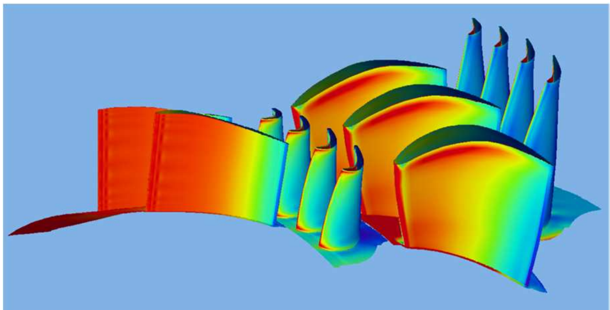
Figure 24. Mach number contours in high pressure two stage turbine
