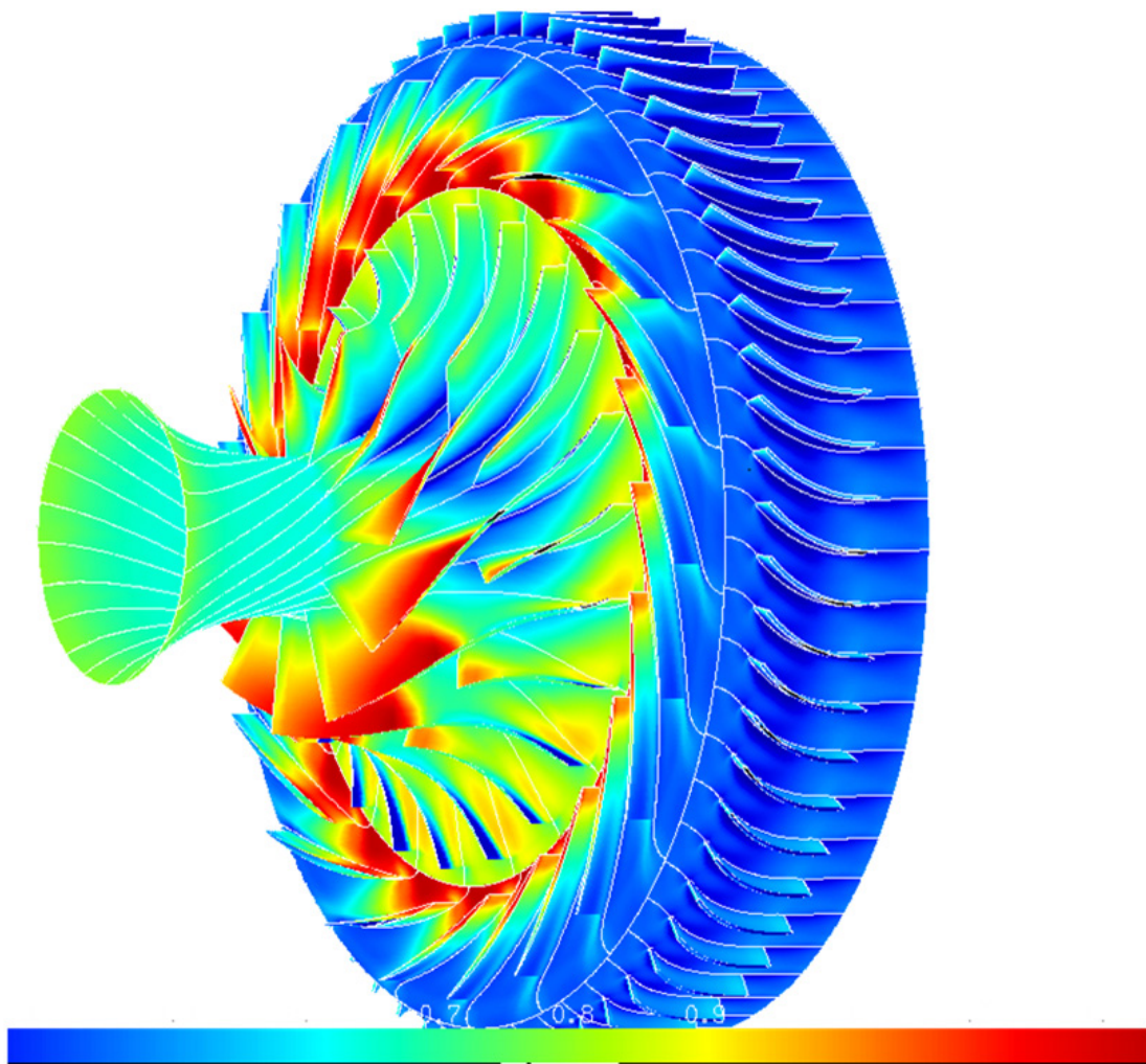
Figure 23. Static pressure distributions in the centrifugal compressor
