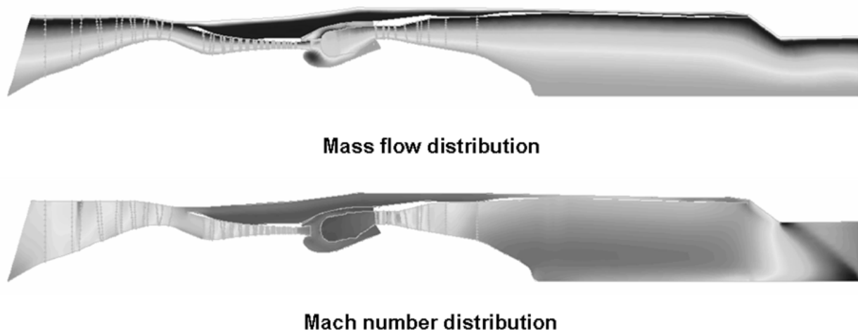
Figure 22. Examples of steady and unsteady calculations in turbojet engine
