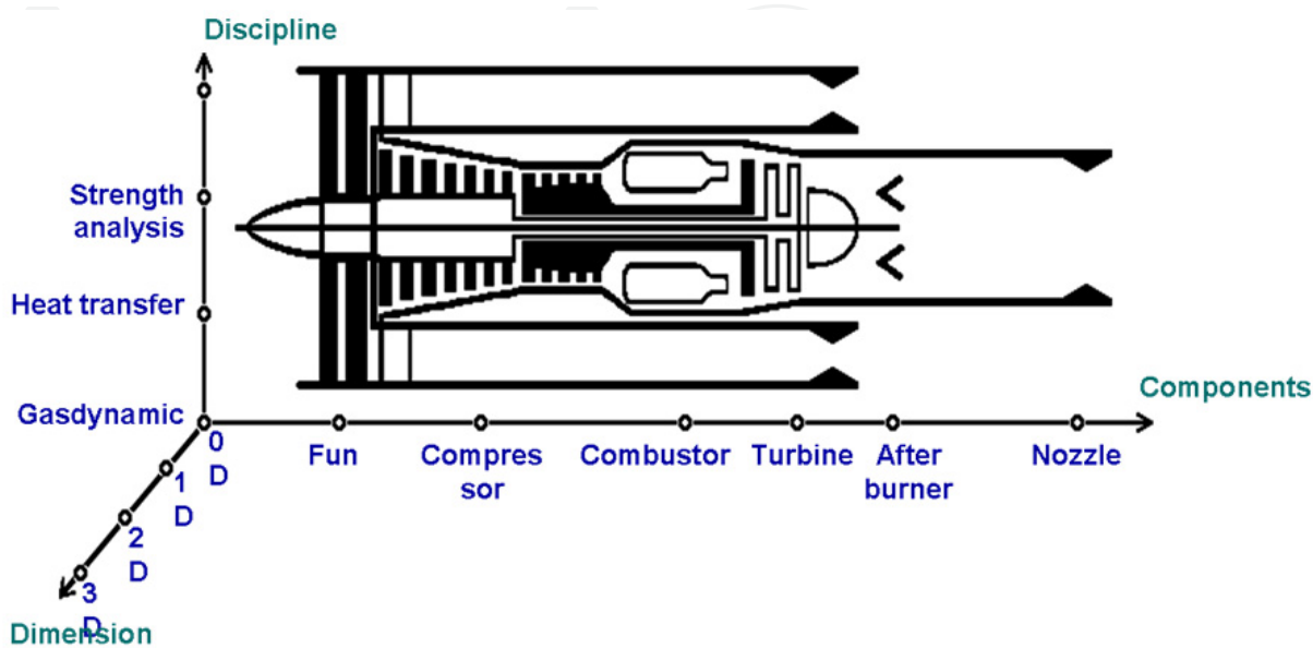
Figure 21. Air Breathing engine scheme (bypass turbojet)
