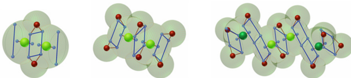
Figure 15. Complex B_2 H_2 and molecules B_2 H_6 and B_4 H_{10}
