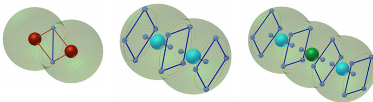
Figure 10. Structures for H_2 , O_2 and CO_2 molecules
