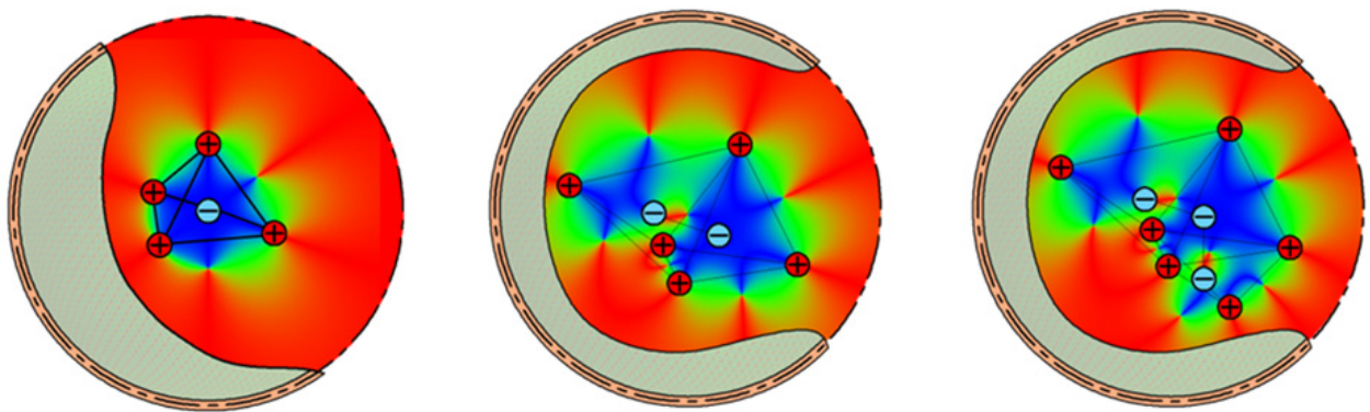
Figure 19. Internal structures of Lithium {}^4\text{Li} , {}^5\text{Li} and {}^6\text{Li}
