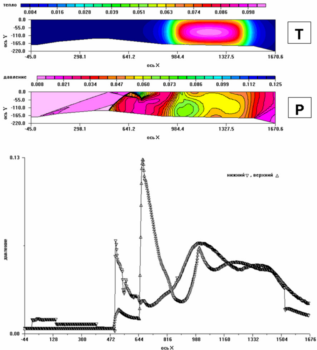
Figure 25. Pressure distributions in channel walls with intensive heat addition
