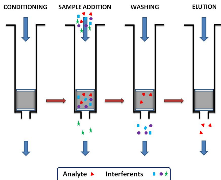
Figure 1. Schematic representation of SPE clean-up procedure.
