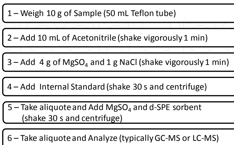
Figure 6. Schematic view of a typical analytical QuEChERS procedure for the analysis of pesticides as described in [75].
