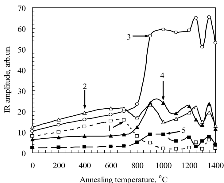
Figure 12. Amplitude of IR transmission for various wavenumber values versus an annealing temperature. (1 - \square ) 700 \text{cm}^{-1} , (2 - \triangle ) 750 \text{cm}^{-1} , (3 - \circ ) 800 \text{cm}^{-1} , (4 - \blacktriangle ) 850 \text{cm}^{-1} , and (5 - \blacksquare ) 900 \text{cm}^{-1} .
