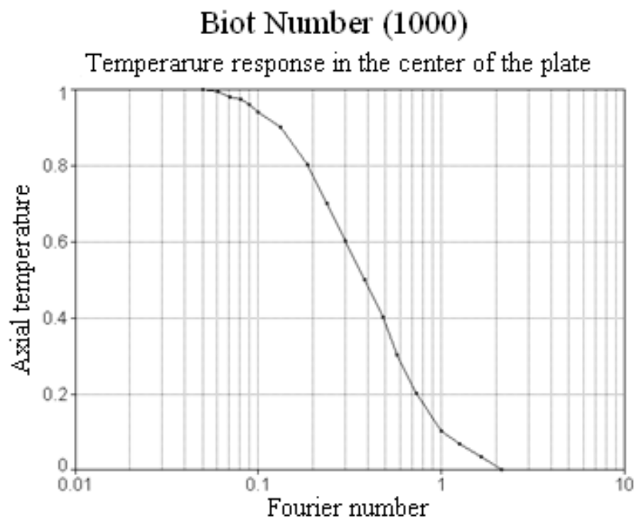
Figure 8. Biot number for infinite plate
