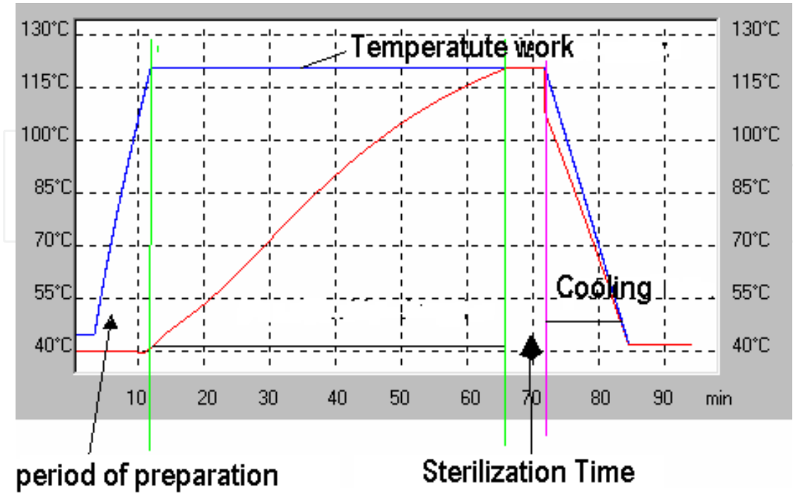
Figure 12. Characteristic line of a process of commercial sterilization
