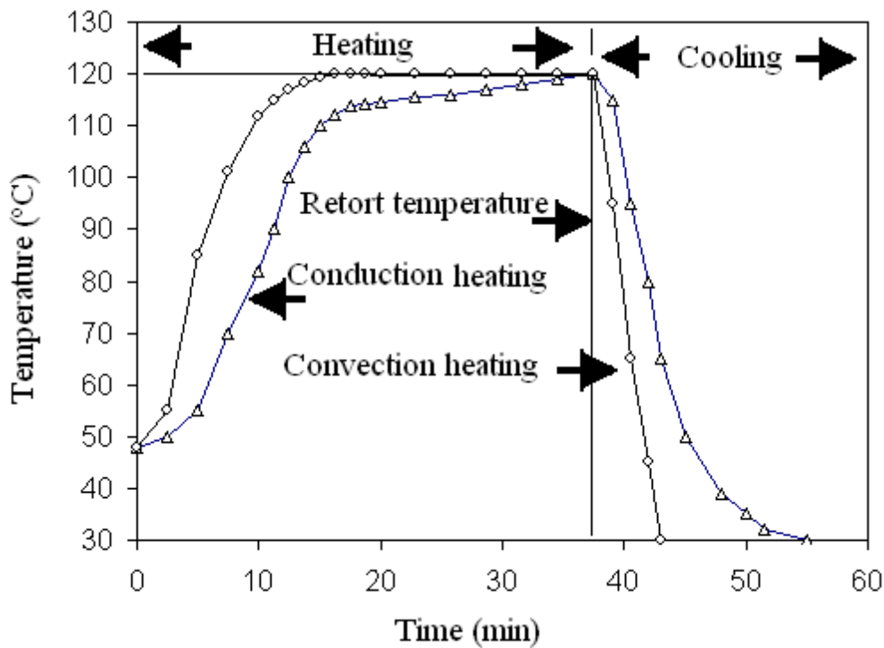
Figure 3. Heat penetration profiles of conduction and convection heating foods.
