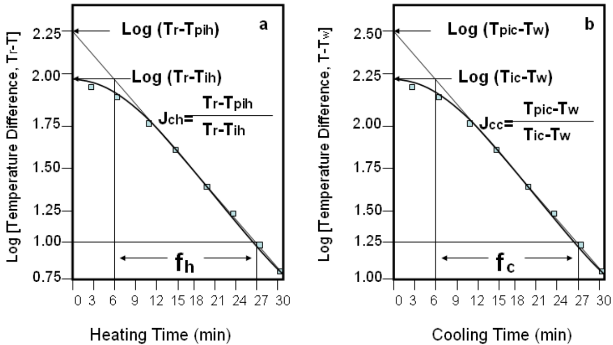
Figure 4. Heating curve and heating parameters (a), cooling curve and cooling parameters (b).
