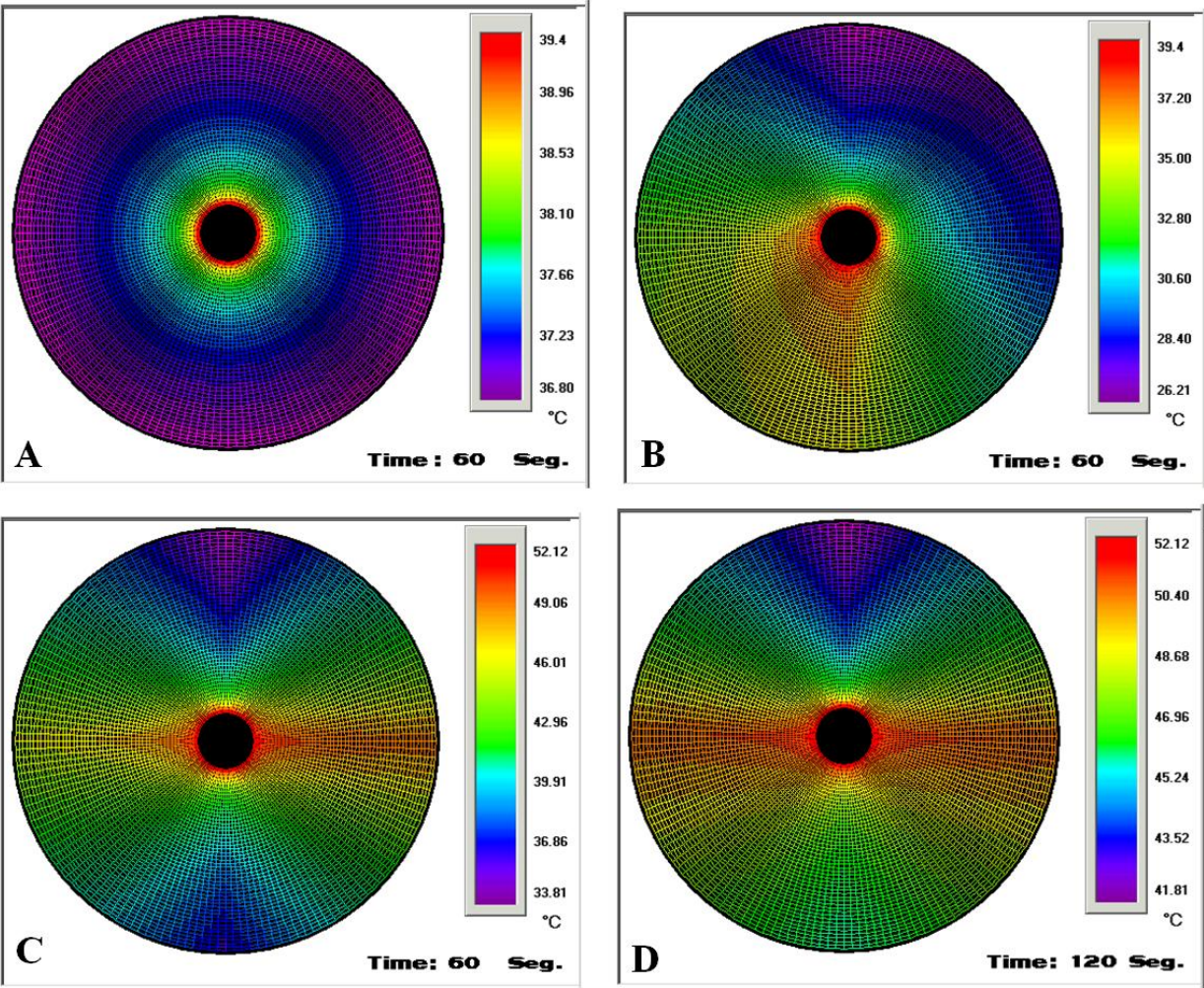
Figure 13. A Theory model, B Real flux heat in apple, C and D Real flux heat in pear
