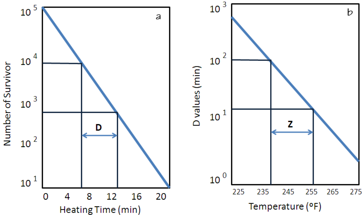
Figure 1. (A) Typical survivor curve. (B) A typical thermal resistance curve.
