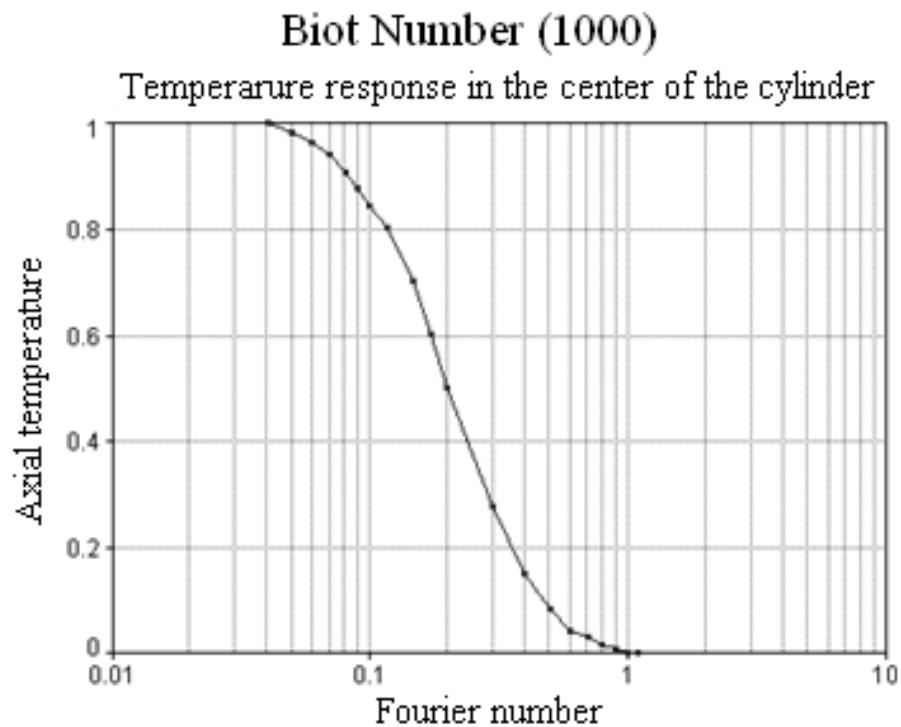
Figure 9. Biot number for Infinite Cylinder
