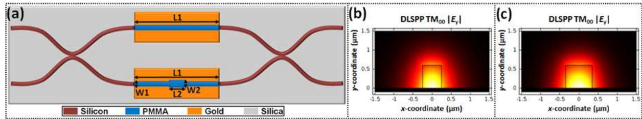
Figure 7. (a) Schematic layout of a Si-DLSP A-MZI. The lower plasmonic branch is widened in order to introduce a default asymmetry, (b) fundamental quasi-TM mode of the 500 \times 600 \text{ nm}^2 PMMA-loaded SPP waveguide, (c) fundamental quasi-TM mode of the 700 \times 600 \text{ nm}^2 PMMA-loaded SPP waveguide.
