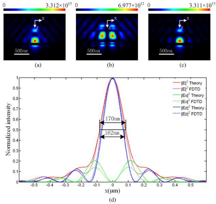
Figure 3. The intensity distribution of radially polarized beam focusing through silver film. Colorbar unit: \text{V}^2/\text{m}^2 . (a) |E_{total}|^2 ; (b) |E_x|^2 ; (c) |E_z|^2 ; (d) Comparison of the sizes of the SPs enhanced focus with that of theoretical normal focus.
