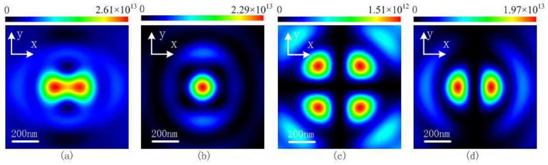
Figure 6. The intensity distribution of evanescent electric field for linearly polarized focal beam at the interface. (a) I = |E_x|^2 + |E_y|^2 + |E_z|^2 (b) |E_x|^2 (c) |E_y|^2 (d) |E_z|^2 (Unit: V^2/m^2 )
