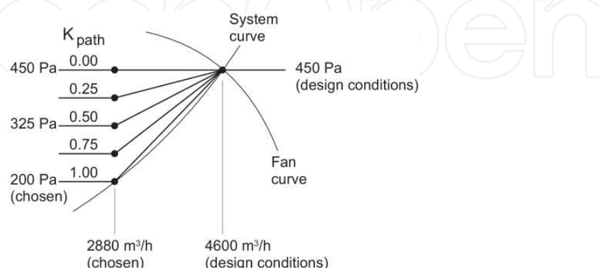
Figure 8. Paths of the pressure difference set point of the fan as a function of the correction gain K_{\text{path}} .
