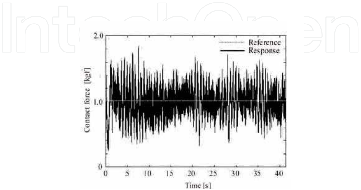
Figure 11. Force control result in playback mode
