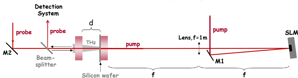
Figure 11. Experimental setup. Two 1 mm-thick ZnTe crystals are used to generate and detect the THz pulse. The pump and probe pulses are delivered by a regenerative amplifier (Coherent Legend) at 800 nm, with 50 fs duration, working at a 1 kHz repetition rate. The pump beam is spatial patterned by a SLM working in reflection. The THz pulse is measured along the propagation direction for different distances d between the generating and detecting crystal. The pump beam is focussed in the generating crystal by means of a 1 m focal lens. The latter also realizes the spatial Fourier transform (taken from [7]).
