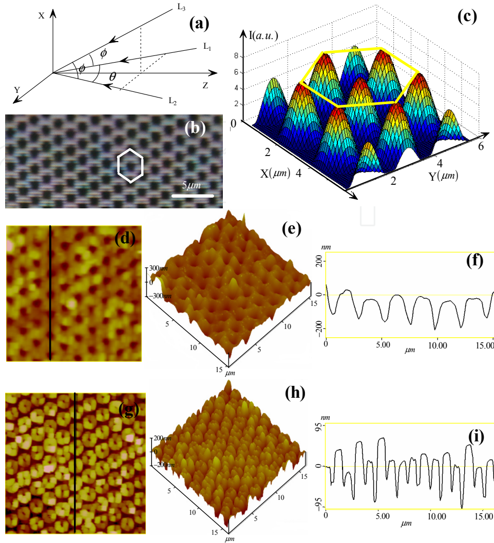
Figure 10. (a) Geometric sketch of the three non-coplanar interfered beams, and the sample is laid in the x - y plane, (b) Photo of the periodic microstructure fabricated in silica glass, taken by an optical microscopy, (c) Calculated intensity distribution of the interference by three non-coplanar beams. The induced periodic microstructure depicted by an AFM: (d) Energy is 75 \mu\text{J} per pulse, (g) Energy is 30 \mu\text{J} per pulse, (f) (i) Three-dimensional image of the microstructure of (d) and (g) respectively, (e) (h) The cross section of the microstructure in the direction of black line showed in (d) and (g) respectively
