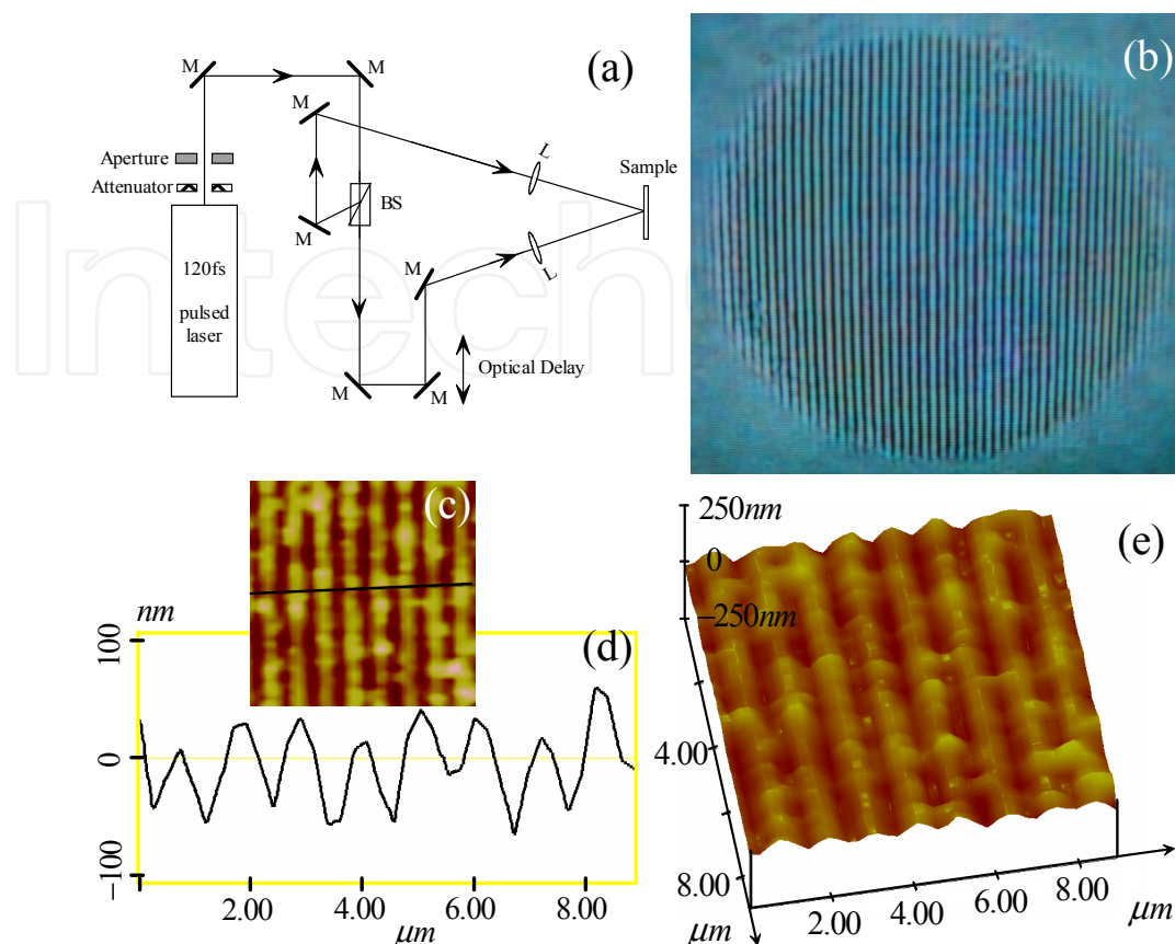
Figure 2. The experimental setup for the holographic fabrication of microgratings, (b) the fabricated grating observed by optical microscopy, (c) top-viewing AFM image of the fabricated grating, (d) cross-section view in the direction of black line shown in (c), (e) three dimensional view of the fabricated structure.
