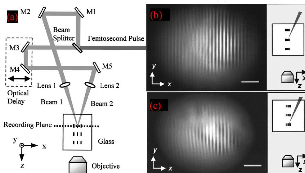
Figure 4. (a) Top view of the experimental setup for the formation of multiple gratings inside glass. The recording plane is in the x-y plane and through the overlapping focal points of the two incident beams: beam 1 and beam 2. (b)(c). Readout images of the second and the third layers of grating inside a slide glass plate by beam 2. The images were taken through a 100X optical objective that was focused onto the recording planes at depths of 400\mu\text{m} (b) and 600\mu\text{m} (c) respectively. The schematics on the right indicate the relative positions of the sample, grating layers, the readout beam, and the 100X optical objective. Scale bar: 5\mu\text{m} .
