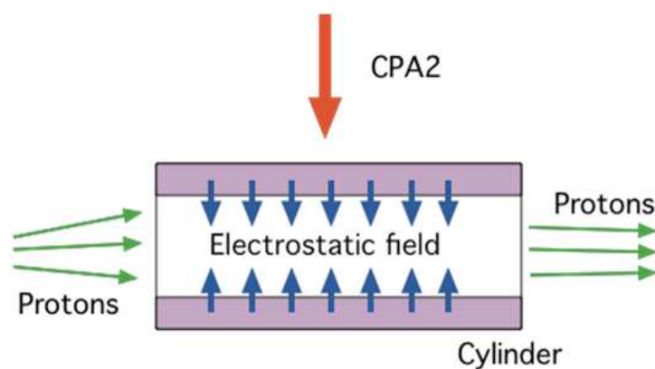
Figure 8. Schematic of the micro-lens setup focalizing a proton beam propagating on its axis. The proton beam is accelerated from a planar metallic foil by a first laser pulse. The proton beam is focalized using the hollow cylinder irradiated on the side by the laser pulse CPA2.
