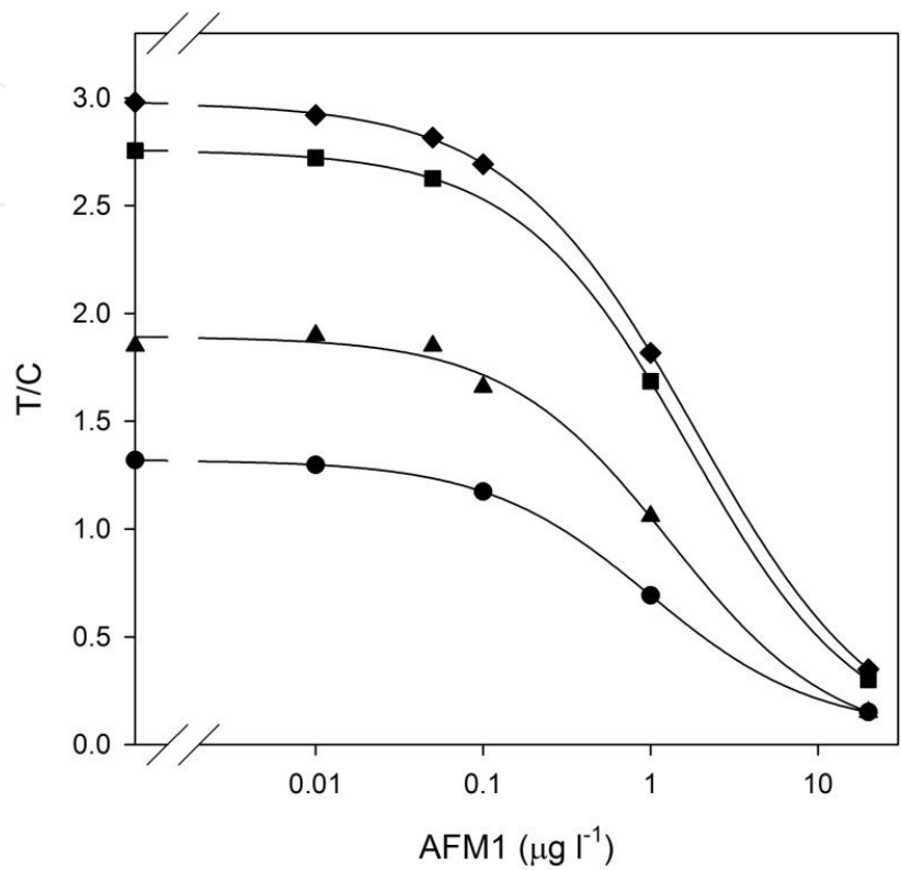
Figure 5. Effect of the amount of antibodies coated onto the GNPs (Ab) compared to the amount needed for saturating GNP surface (Ab SAT ) for varying Ab/ Ab SAT : 0.5 (■), 0.7 (▲), 1 (●), 1.5 (◆). GNP-antibodies dispensed at OD 3; T-line: AFM 1 -BSA conjugate (0.2 mgml -1 , SR=22).
