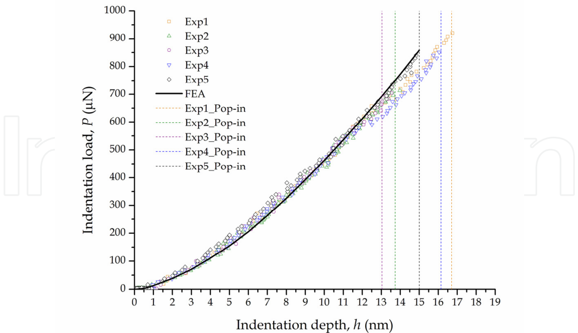
Figure 6. Measured load-displacement curves for all analyzed indentation experiments using the blunt indenter and the corresponding FEA-simulated pop elastic deformation curves using the AFM-measured indenter. The dotted lines indicate the major pop-in location for each experiment.
