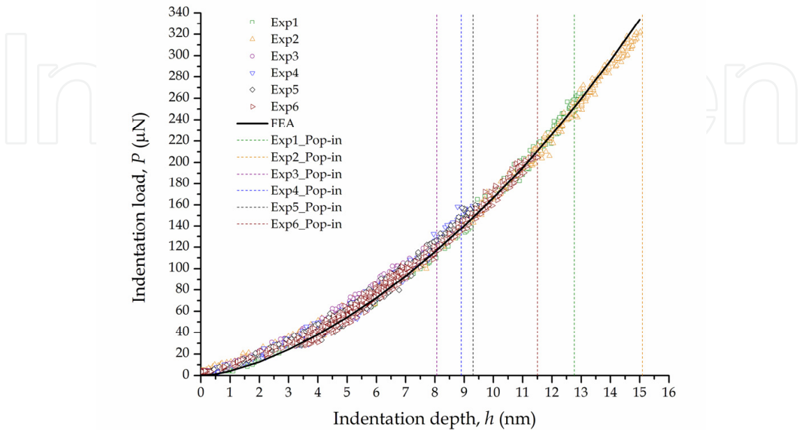
Figure 5. Measured load-displacement curves for all analyzed indentation experiments using the sharp indenter and the corresponding FEA-simulated elastic deformation curves using the AFM-measured indenter. The dotted lines indicate the major pop-in location for each experiment.
