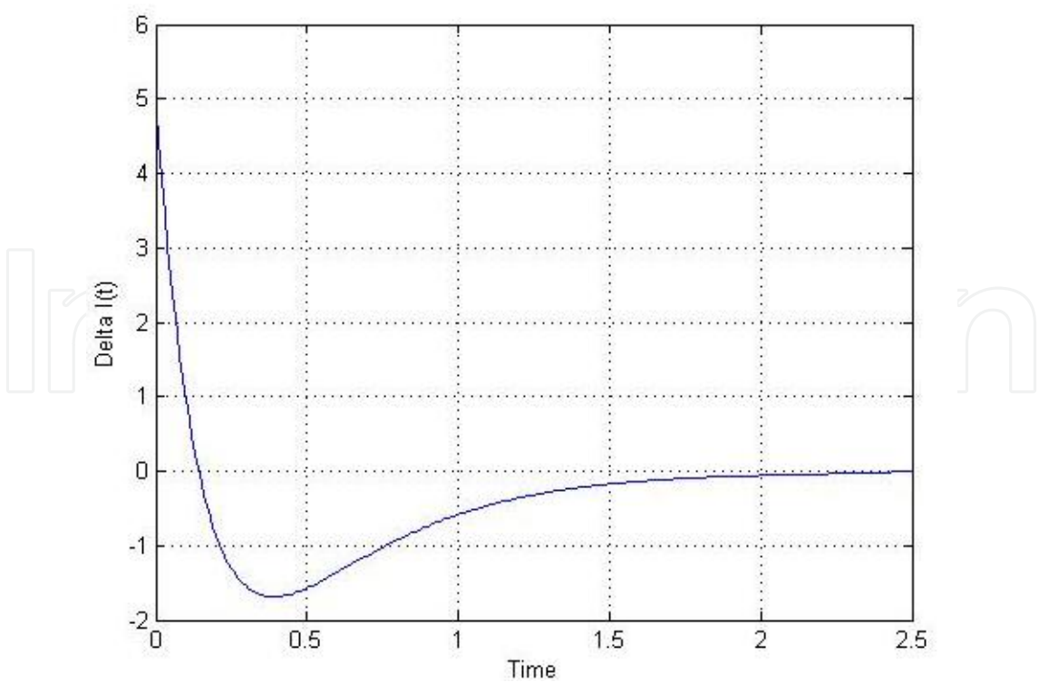
Figure 1. Variation of the optimal inventory level
