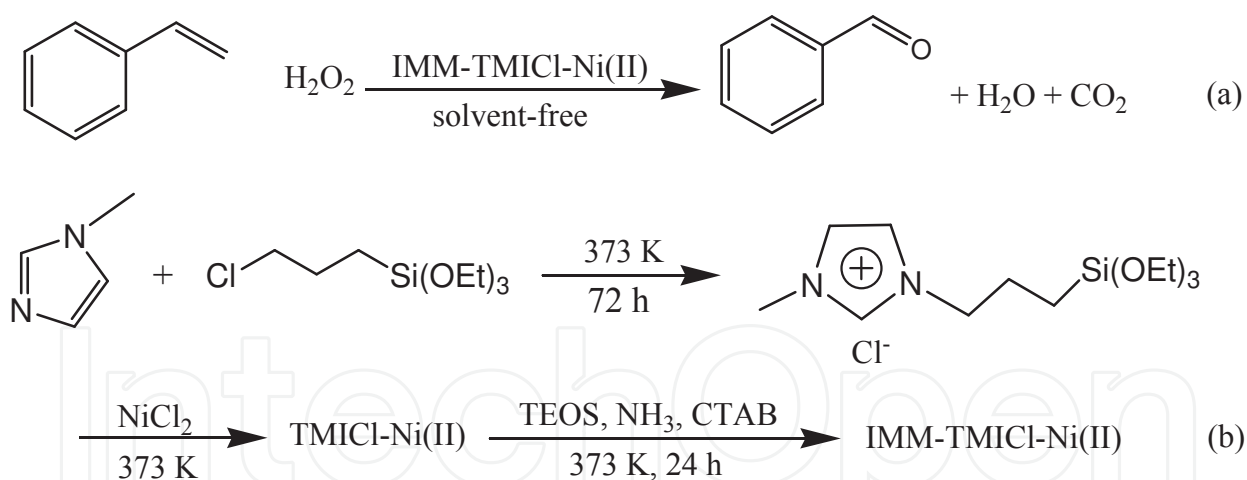
Figure 9. Schematic illustrations of (a) oxidation of styrene to benzaldehyde with \text{H}_2\text{O}_2 under solvent-free condition, (b) synthesis of IMM-TMCl- \text{Ni}(\text{II}) catalyst by grafting \text{Ni}^{2+} on IL-Silica. [53]
