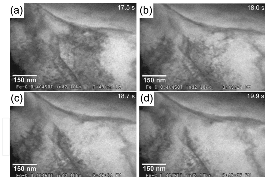
Figure 9. In situ TEM micrographs of the Fe–0.4C martensite showing details of the “sink” of dislocations at the high-angle grain boundary. Frames (a–d) correspond to a sequence between Figs. 8(c) and 8(d). Penetration depth increases from (a) to (d).
