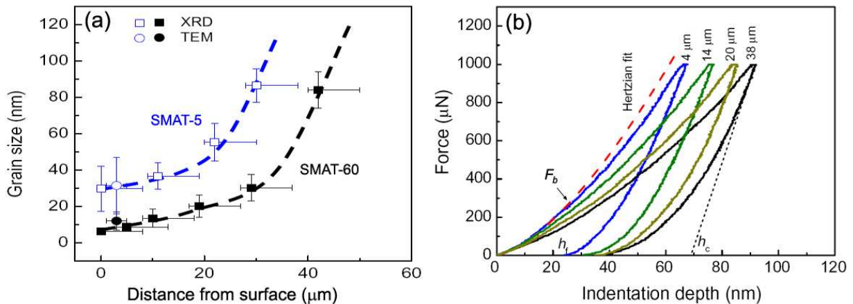
Figure 13. (a) Variation in grain size with distance from the surface for SMAT samples. (b) Typical force-indentation depth curves at different distance D for SMAT-60 as indicated. Definition of the bifurcating force F_b , h_c and h_f are indicated.
