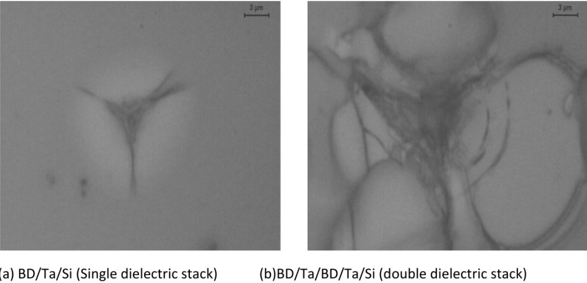
Figure 9. Optical micrographs of residual nanoindentation impression on single and double dielectric stacks.
