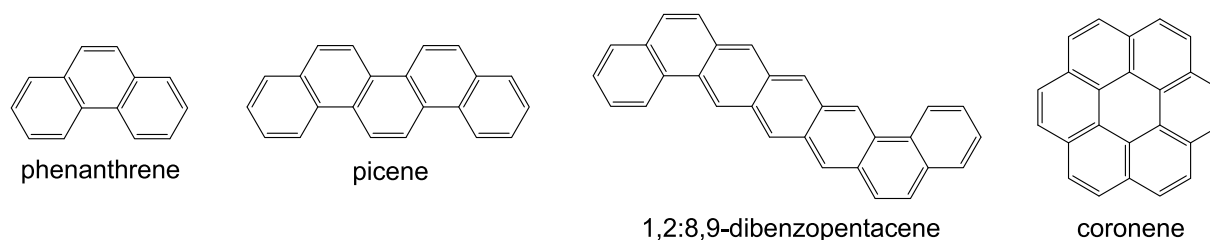
Scheme 8.
