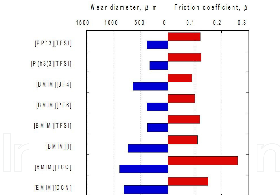
Figure 3. Lubricity of each ionic liquid for steel/steel sliding
