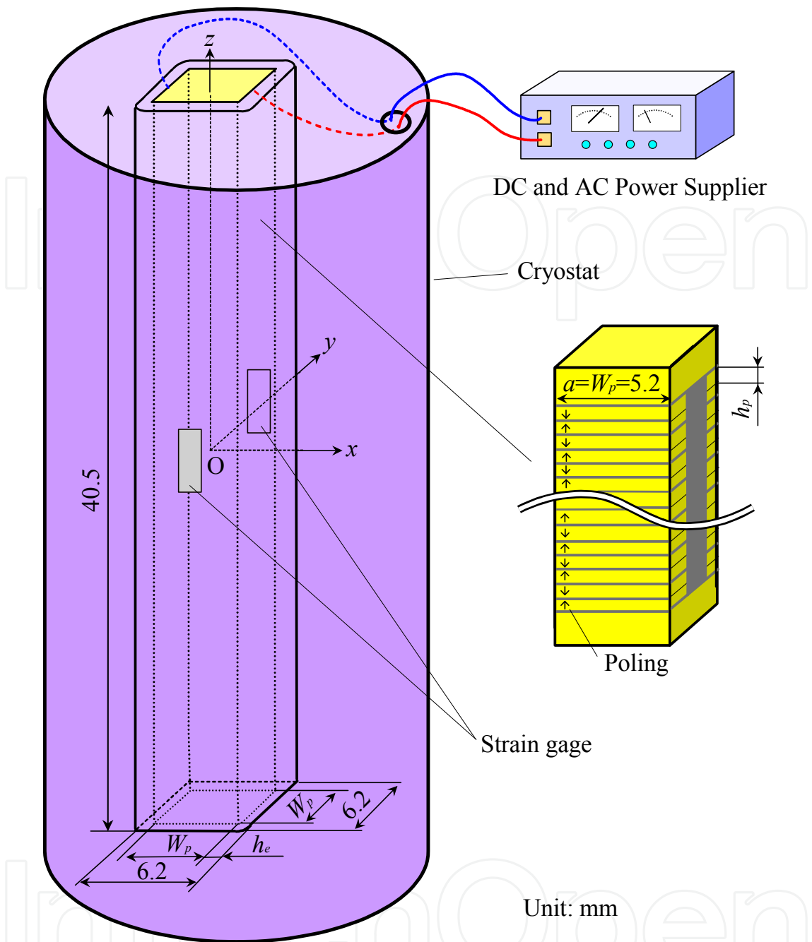
Figure 6. Experimental setup.
