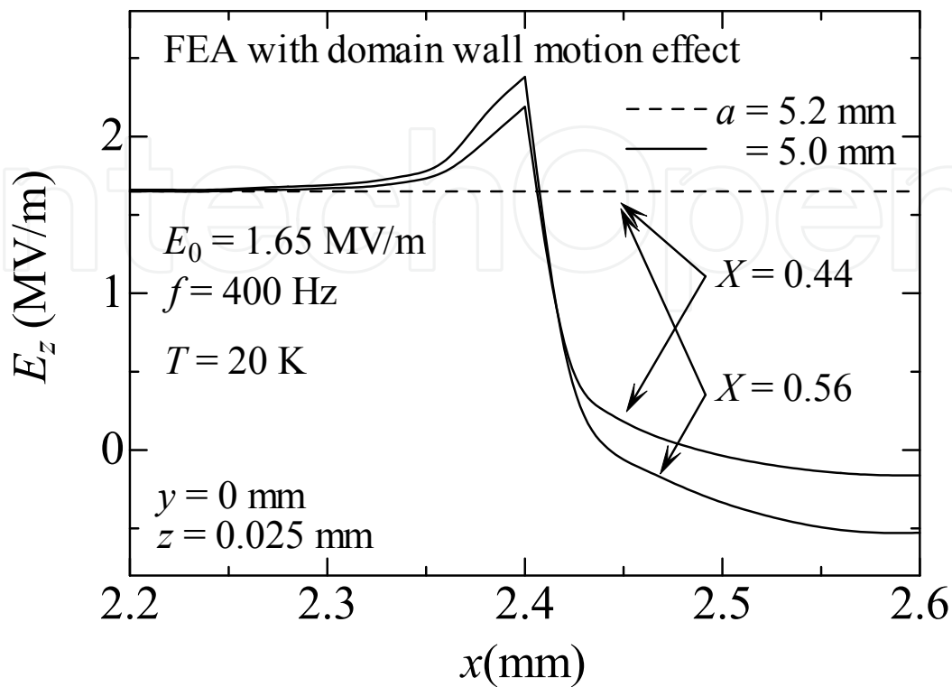
Figure 12. Variation of electric field E_z as a function of x at y = 0 mm and z = 0.025 mm for PZT stack actuators under E_0 = 1.65 MV/m at T = 20 K.
