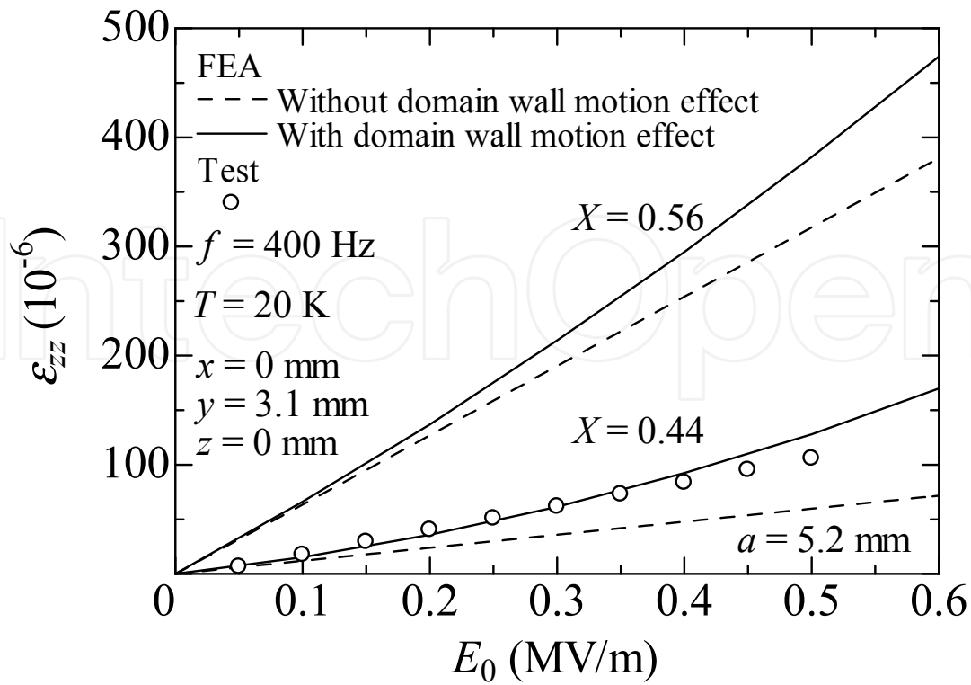
Figure 10. Strain vs AC electric field of PZT stack actuators for X = 0.44 and 0.56 at 20 K.
